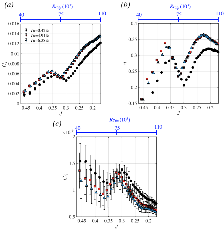
Fig. 8 (a) The coefficient of thrust ( C_T ), (b) efficiency ( \eta ) and (c) the coefficient of torque ( C_Q ) for the rotor in the climbing configuration for a fixed U_o = 3.5 m/s varying the rotation speeds from 2000–5000 RPM for the three upstream flow configurations.
