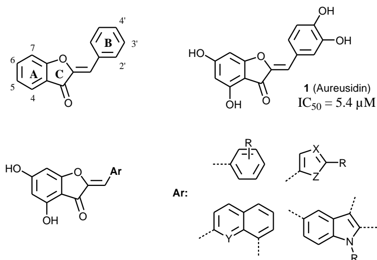
Fig. 1. General structure of the aurone backbone (top left), structure and activity of the naturally occurring aureusidin 1 and structures of aurone derivatives investigated in this study (the dashed line indicate the site of linkage).
