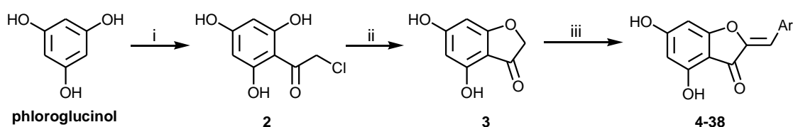
Scheme 1. General pathway for the synthesis of aurone derivatives. Reagents and conditions: (i) ClCH 2 CN, HCl, ZnCl 2 , Et 2 O, 0°C; (ii) H 2 O, 100°C, 5 h, 84 % (for 2 steps); (iii) ArCHO, KOH 50% in H 2 O, EtOH, reflux, 2-15 h.
