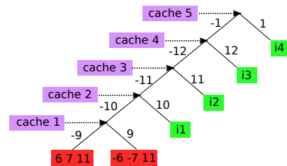
Figure 5: Search tree for marg2x2.cnf with caching.
