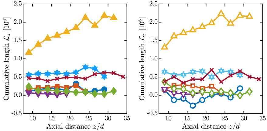
FIG. 11. Cumulative length \mathcal{L}_z of quantized vortices per unit height as a function of the normalized axial distance z/d . Left panel: right-hand side of Eq. (15), computed using the experimentally obtained values of L_0 and w . Right panel: result of the numerical integration of the right-hand side of Eq. (11) as discussed in the text. Colors as in Fig. 9.
