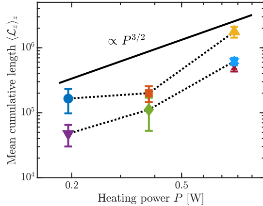
FIG. 12. Mean cumulative length \langle \mathcal{L}_z \rangle_z as a function of the heating power P . Colors as in Fig. 9; error bars correspond to one standard deviation interval. Black dotted lines connect data points collected at the same temperature of the helium bath.
