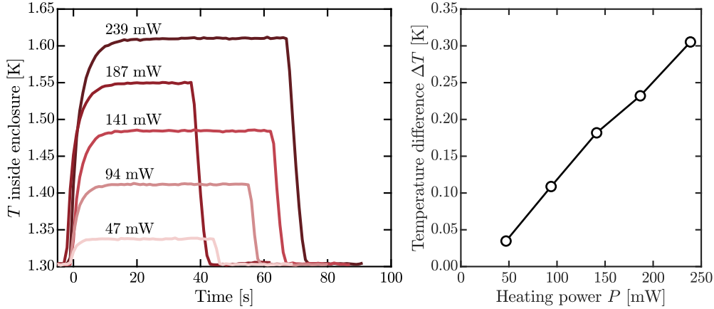
FIG. 6. Left panel: temperature inside the heater enclosure as a function of time. The bath temperature is kept constant at 1.30 K and the heater is supplied by a constant heating power (specified near each curve) from approximately zero time. Right panel: steady temperature difference \Delta T between the enclosure and the ^4\text{He} bath as a function of the heating power P .
