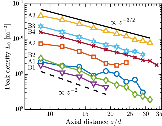
FIG. 9. Peak vortex line density L_0 as a function of the normalized axial distance z/d . Data set labels are indicated to the left of each curve. Note the log-log scale.
