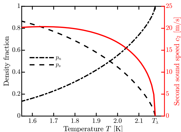
FIG. 1. Left axis: temperature dependence of the density fractions of the normal ( p_n , dot-dashed line) and superfluid ( p_s , dashed line) components of He II. Right axis: temperature dependence of the second sound speed (solid line). T_\lambda \approx 2.2 K denotes the superfluid transition at the saturated vapor pressure. Data from Ref. ? .
