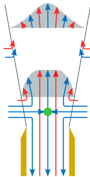
FIG. 2. Sketch of the two-component flow field in a thermal counterflow jet. Red (blue) arrows: normal (superfluid) component; green point: stagnation point of the superfluid component. Displayed are also velocity profiles in the near field, i.e. in the close proximity of the nozzle (bottom) and in the intermediate field (top), see Eq. (??). Adapted from Ref. ? .
