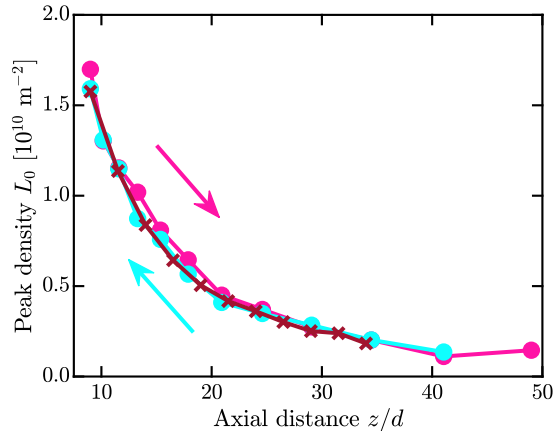
FIG. 8. Peak vortex line density (i.e. density along the jet axis) L_0 as a function of the axial distance z , normalized by the nozzle diameter d , for data sets B4 (red crosses) and C1 (cyan and magenta points). Color arrows denote the direction of the sensor stroke (receding from or approaching towards the nozzle).
