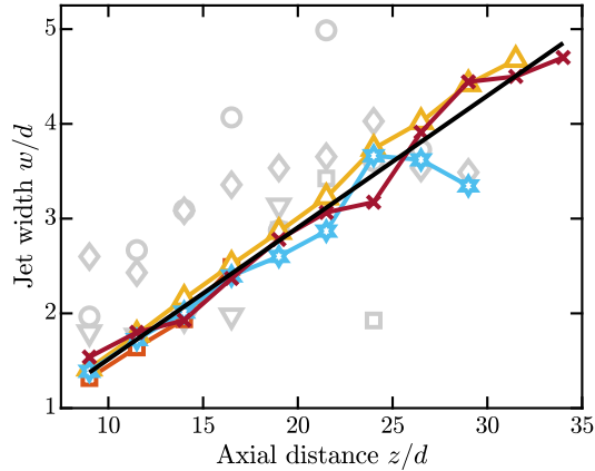
FIG. 10. Peak width w as a function of the axial distance z (both quantities are normalized by the nozzle diameter d ). Color symbols: points with L_0 > L_t , i.e. data sets A2 (in part), A3, B3, and B4, collectively named high set; gray symbols: remaining points, with L_0 \leq L_t , i.e. data sets A1, A2 (in part), B1 and B2, collectively named low set. Note that the symbols are as in Fig. ??, regardless of their color; black line: linear fit, Eq. (??).
