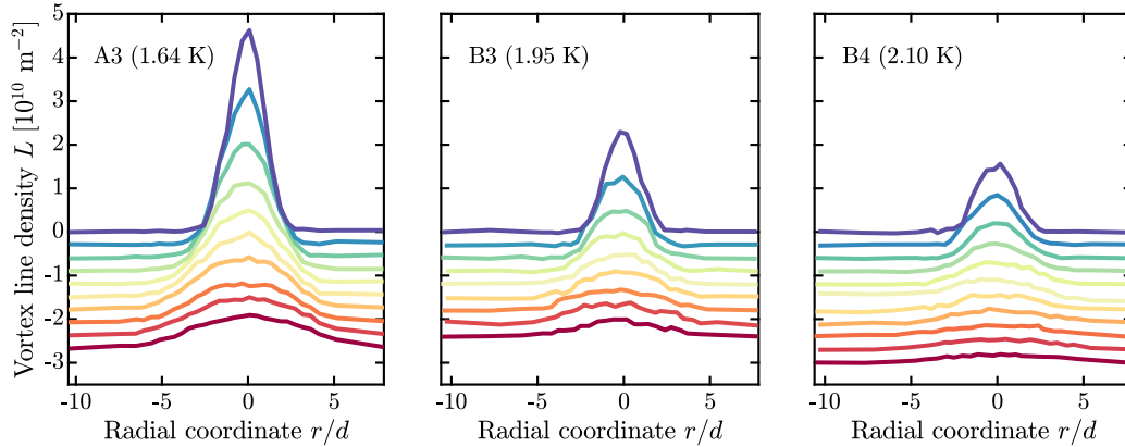
FIG. 7. Radial profiles of the vortex line density for P \approx 776 mW and different temperatures. The colors correspond to different axial positions of the sensor, from 9d above the nozzle (dark blue) to 31.5d , 29d and 34d (dark red) for the left, middle and right panels, respectively, with steps of 2.5d . The curves are offset by 3 \times 10^9 m ^{-2} for the sake of clarity. Positive and negative values of the radial coordinate r , here normalized by the nozzle diameter d , denote the corresponding angular deflection ( r/d < 0 means \alpha < \alpha_0 and vice versa).
