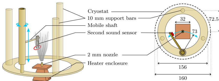
FIG. 3. Sketch of the experimental setup (not to scale). Brown: 3D-printed heater enclosure; blue arrows: possible motions of the mobile shaft; red: sensitive area of the second sound sensor. Dimensions in the right panel are in millimeters.
