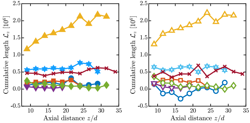
FIG. 11. Cumulative length \mathcal{L}_z of quantized vortices per unit height as a function of the normalized axial distance z/d . Left panel: right-hand side of Eq. (??), computed using the experimentally obtained values of L_0 and w . Right panel: result of the numerical integration of the right-hand side of Eq. (??) as discussed in the text. Colors as in Fig. ??.
