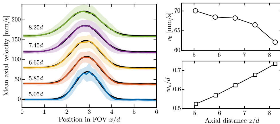
FIG. 5. Left panel: mean axial velocity of our solid particles, visualized in five regions, 0.8d high, crossing the jet axis (the curves are offset by 40 mm/s relative to each other). The distance separating each region center from the nozzle is specified next to each curve. A positive velocity indicates that the particles move, on average, away from the nozzle. Color lines: experimental data; pale color areas: one standard deviation intervals; black lines: Gaussian fits, Eq. (??); see also Sec. ??). Right panels: centerline velocity v_0 (top panel) and jet width w_v (bottom panel) as a function of the distance z from the nozzle, obtained from the Gaussian fits. Note that the quantities x , w_v and z are normalized by the nozzle diameter d .
