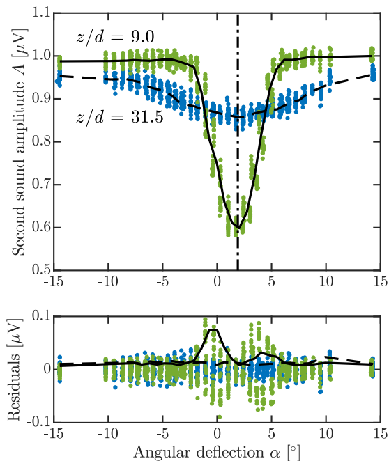
FIG. 4. Top panel: two sets of 30 sweeps (points) across the jet axis, obtained at 1.65 K and 776 mW (data set A3) for z/d = 9.0 and 31.5 , as indicated in the figure. Solid and dashed black lines: ensemble-averaged data used for the calculation of the quantized vortices' density. Dot-dashed black line: deflection offset \alpha_0 \approx 1.9^\circ , Eq. (??). Bottom panel: residuals (points) and standard deviations (lines) corresponding to the data displayed in the top panel.
