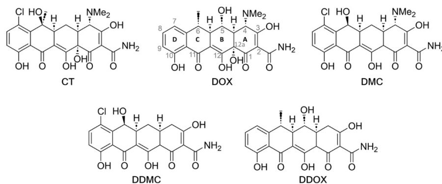
Figure 3. TCs tested in this study. Conventional numbering of the condensed rings and key positions are shown for DOX . The four rings of the TC core structure are designated by A,B,C,D.
