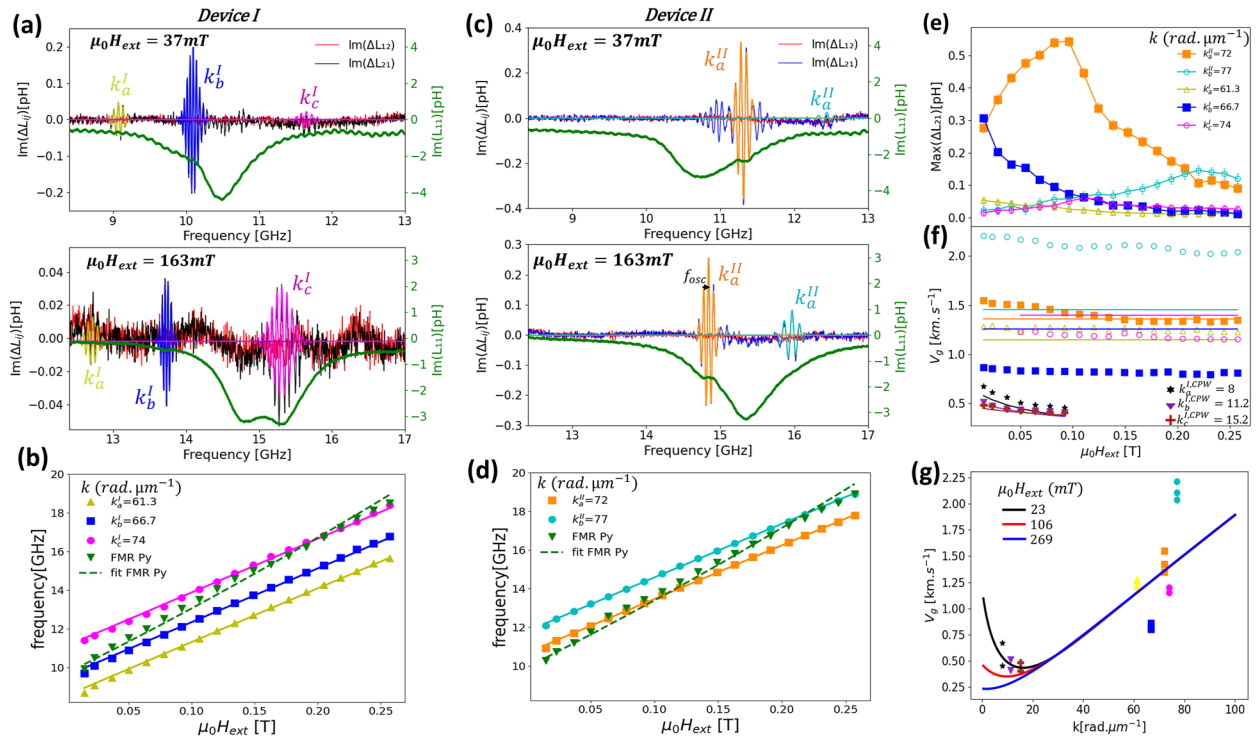
FIG. 3. Transmission spectra at 37 mT and 163 mT for (a) device I and (c) device II, blue and red line represent respectively transmission spectra \Delta_{L_{21}} and \Delta_{L_{12}} . Field dependence of the frequency for the several mode of (b) device I and (d) device II. (e) Field dependence of all the mode amplitudes. (f) and (g) Comparison of the measured group velocity with theoretical expression.
