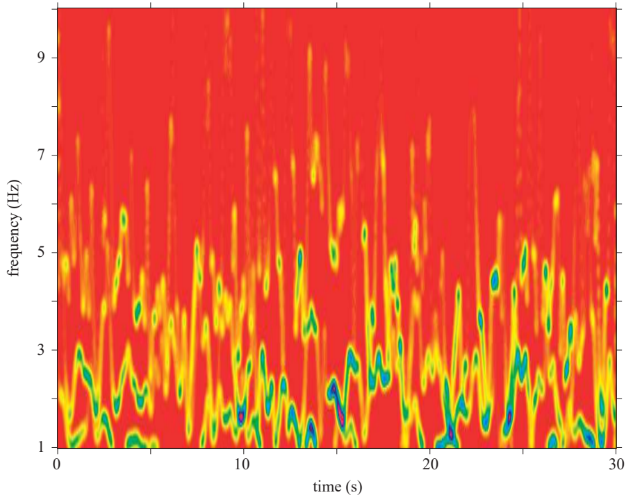
Figure 82. The special Hilbert spectrum with only the energy-containing IMFs ( c_2-c_6 ). The turbulent flow is dominated by the intermittence and frequency modulations, a sure sign that nonlinear mechanisms are at work.
