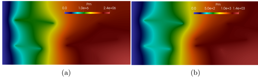
Fig. 3: Matrix overpressures (compared with the initial pressure) in Pa for the reference solution computed on the mesh m = 3 at times t = T/4 (a) and t = T (b) .
