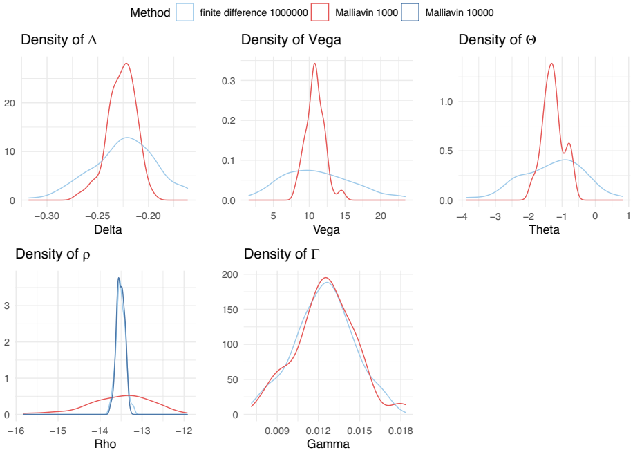
Fig. 2 Densities of simulated \Delta \mathcal{V} , \Theta , \rho , and \Gamma for a digital Asian put option
