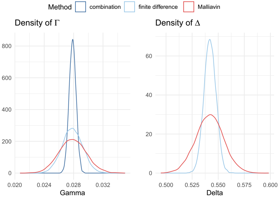
Fig. 1 Densities of simulated \Delta and \Gamma for an Asian call option
