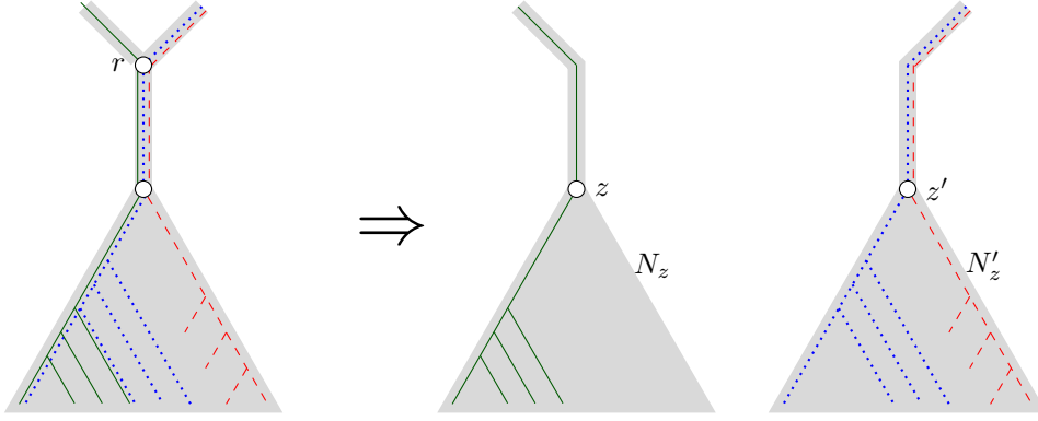
Figure 4. Illustration of the operation of “unzipping” (N, \phi) at a lowest reticulation. The embedding of the three caterpillars X_i, Y_i and Z_i is depicted as green solid, red dashed and blue dotted lines, respectively, within the network outlined in gray. Note that all leaves of N_z into which \phi embeds leaves of X_i as well as at least one of Y_i and Z_i , are duplicated in the process. Note also that not all three caterpillars are necessarily embedded in N_z , as previous unzip operations may have split a caterpillar off N_z .
