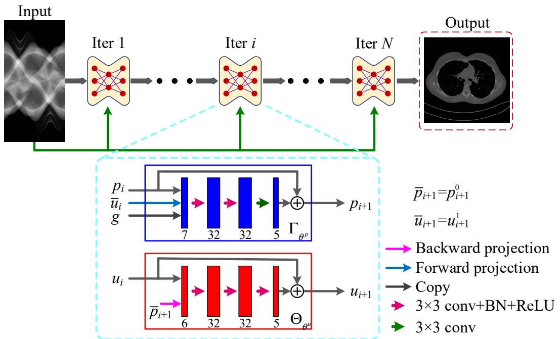
SUP. 2. The network architecture of the Primal-Dual-ReLU.
