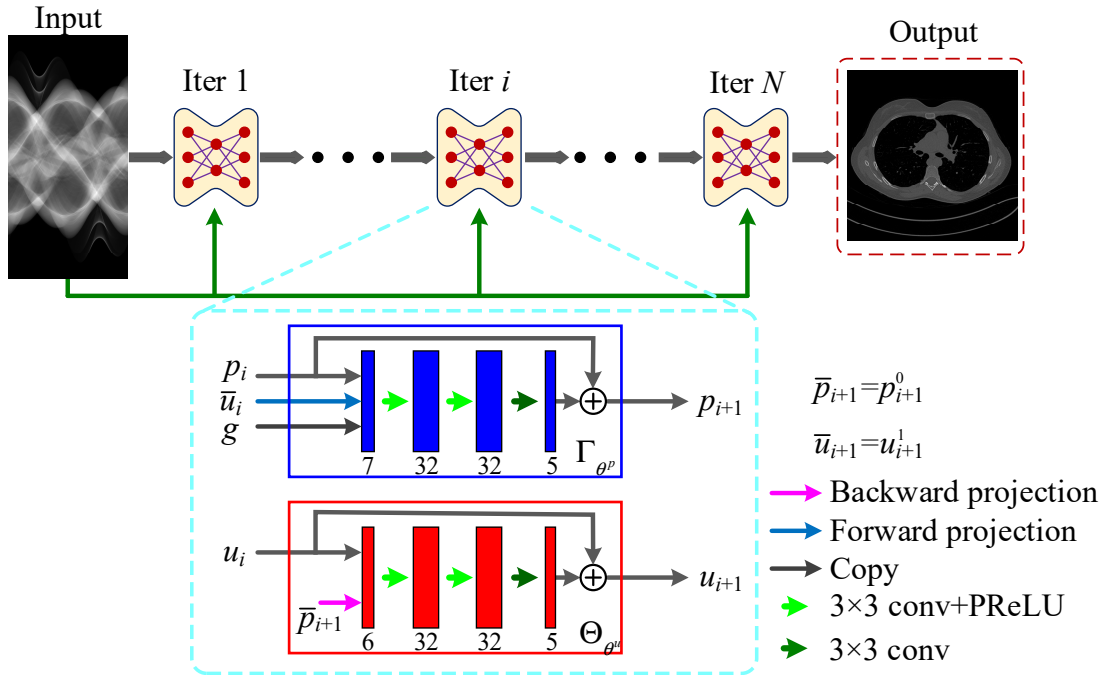
SUP. 1. The network architecture of the Learned Primal-Dual.
