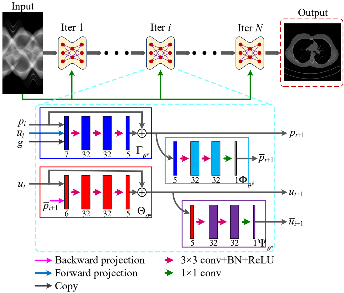
SUP. 3. The network architecture of the Primal-Dual-Fusion.
