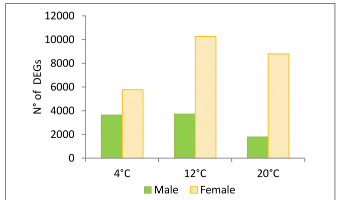
FIGURE 2 | Total number of significant differentially expressed genes (DEGs) (Deseq2, p < 0.001 ; \log_2\text{FC} > 2 , n = 3 ) in Saccharina latissima gametophytes. Up-regulated DEGs in male compared to female gametophytes are indicated in green, and orange in diagonal stripes bars, respectively.
