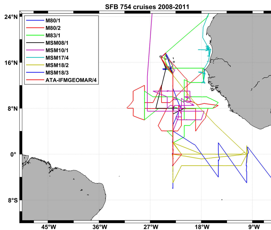
FIGURE 2 | Cruise tracks of nine SFB 754 cruises in the Atlantic Ocean in the first funding period of the project (2008–2011).
