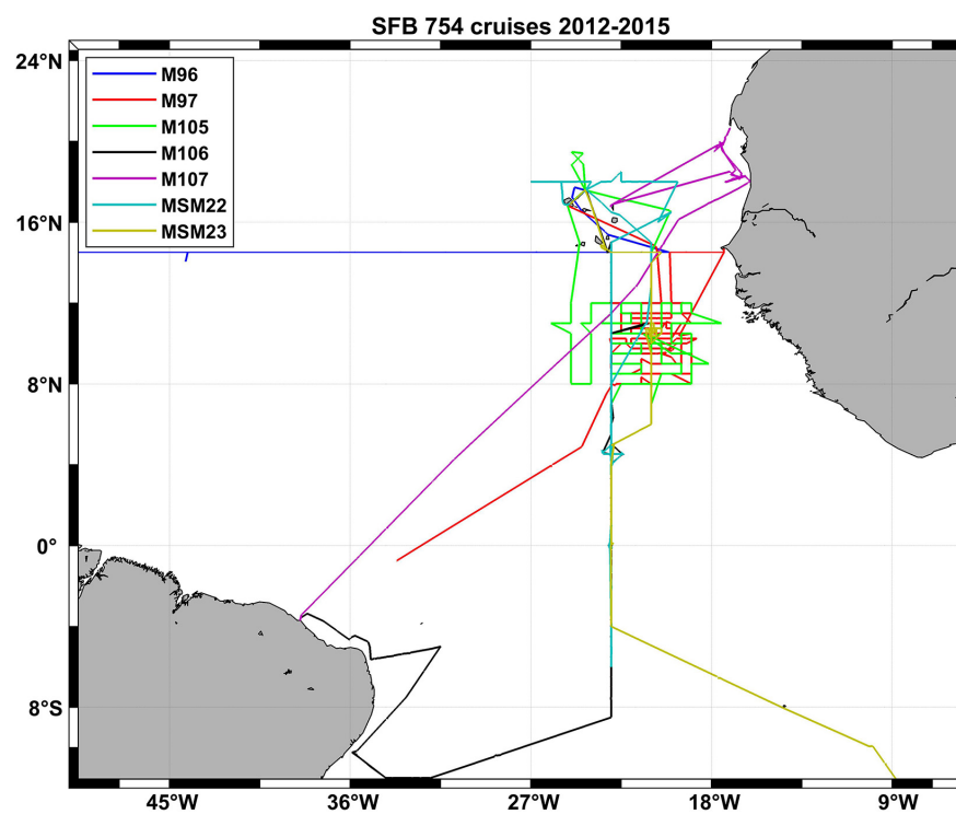
FIGURE 3 | Cruise tracks of seven SFB 754 cruises in the Atlantic Ocean in the second funding period of the project (2012–2015).
