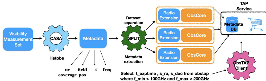
Figure 1. The SPLIT procedure represents a MS dataset as a collection of members datasets whose coverage in spatial and spectral features in ObsCore is compact.
