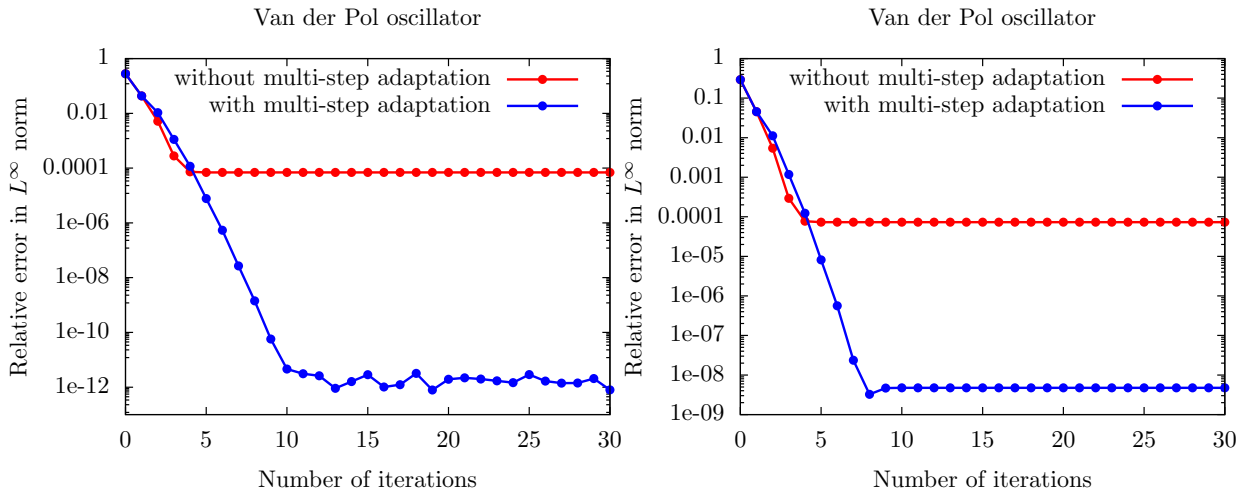
FIGURE 3. Convergence of the multi-step parareal for the third-order BDF method, \delta t = 10^{-4} (left: error (34), right: error (35))
