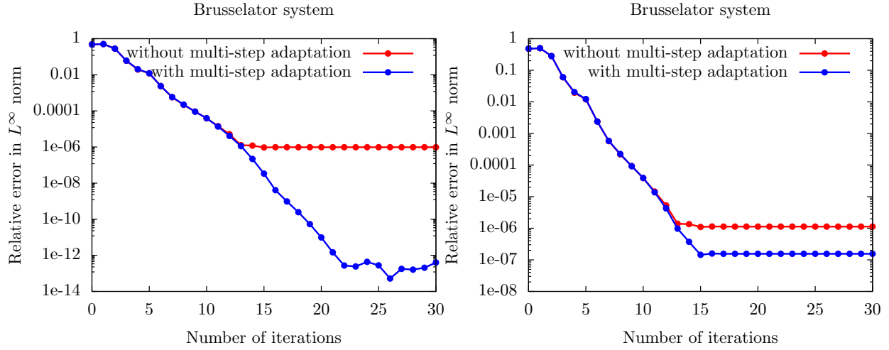
FIGURE 1. Convergence of the multi-step parareal for the second-order BDF method, \delta t = 10^{-4} (left: error (34), right: error (35))
