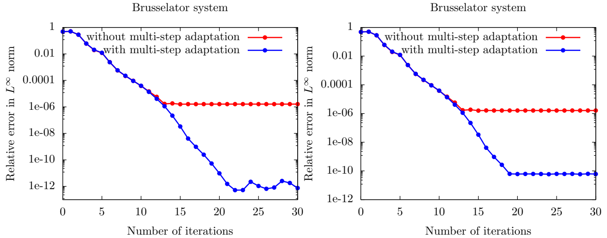
FIGURE 2. Convergence of the multi-step parareal for the third-order BDF method, \delta t = 10^{-4} (left: error (34), right: error (35))
