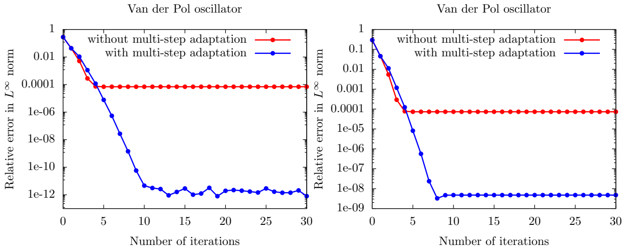
FIGURE 3. Convergence of the multi-step parareal for the third-order BDF method, \delta t = 10^{-4} (left: error (34), right: error (35))
