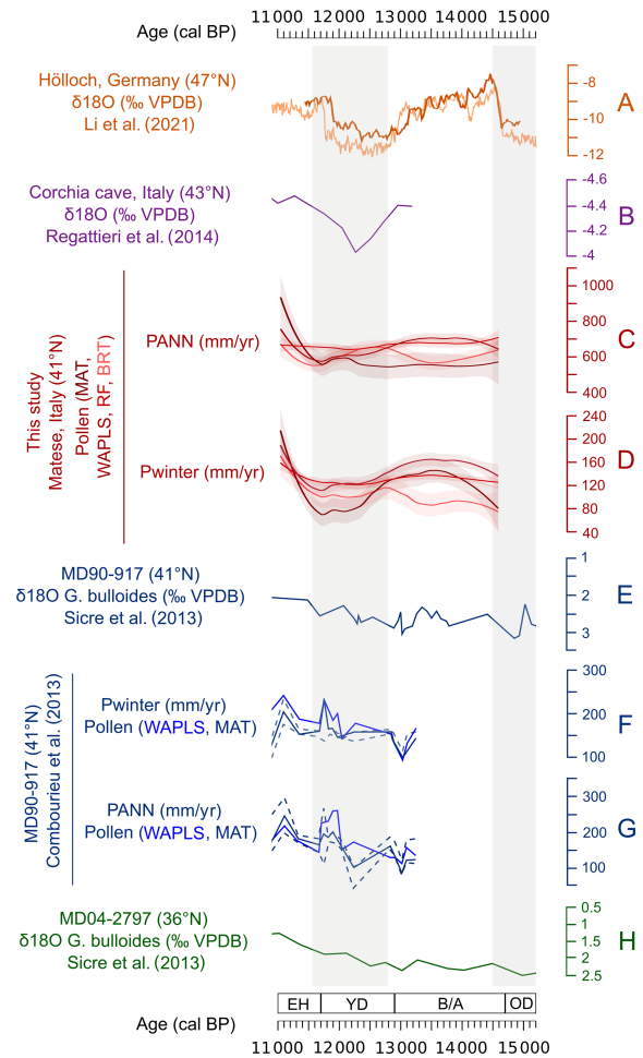
Figure 10. Synthesis of precipitation records inferred from different proxies in Italy from 15 000 to 11 000 cal BP. PANN stands for mean annual precipitation. P_{\text{winter}} is winter precipitation. OD stands for Oldest Dryas. B/A stands for Bølling–Allerød. YD stands for Younger Dryas. EH stands for early Holocene.
