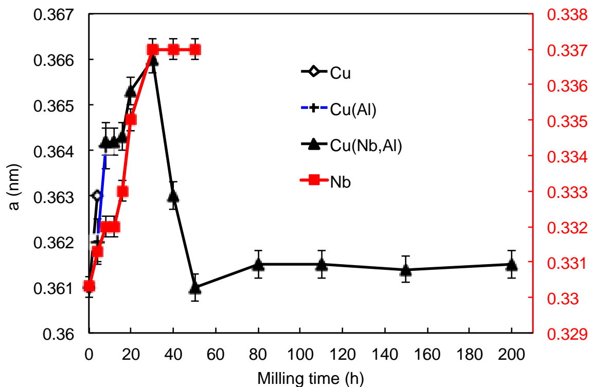
Fig. 7. Lattice parameter evolution as a function of the milling time. The Nb lattice-parameter values are reported on the secondary vertical axis.
