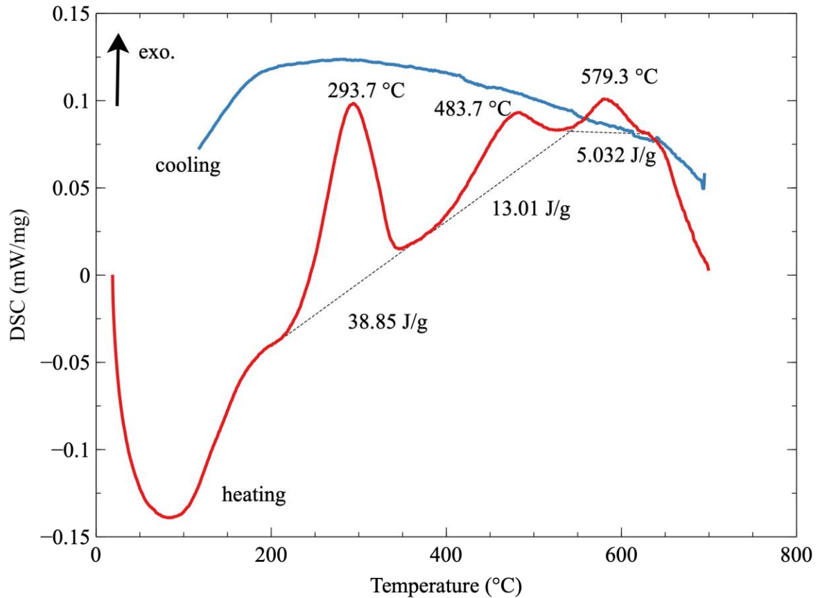
Fig. 11. Typical DSC scans for Cu 70 Nb 20 Al 10 alloy after 200 h of milling at a heating rate of 10°C/min.
