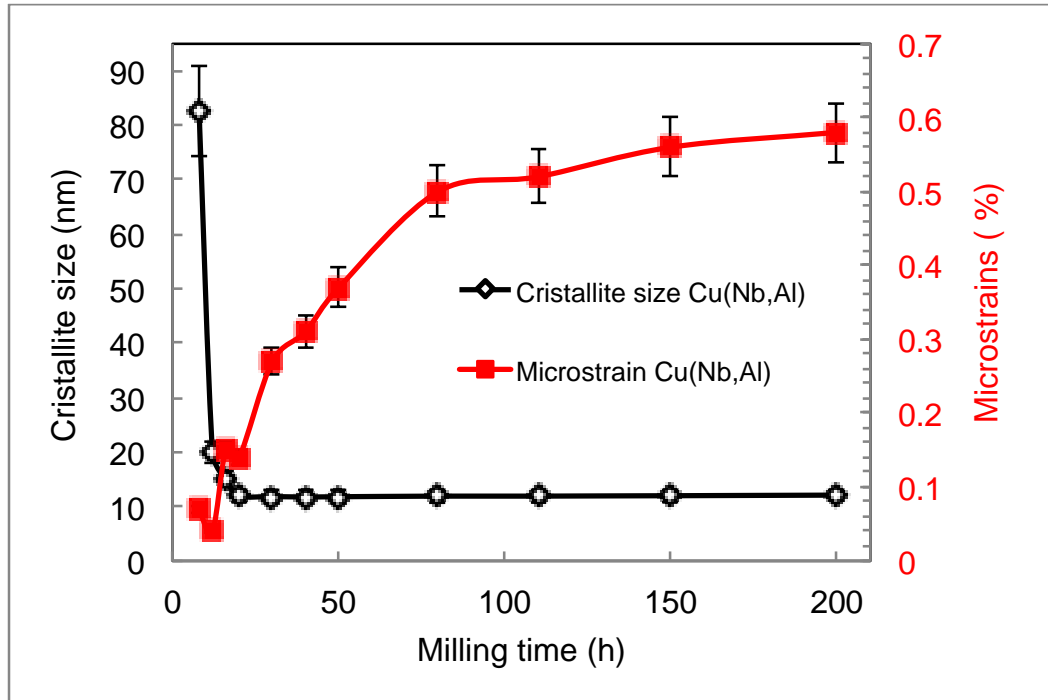
Fig. 8. Evolution of the microstructure parameters of the FCC-Cu(Nb,Al).
