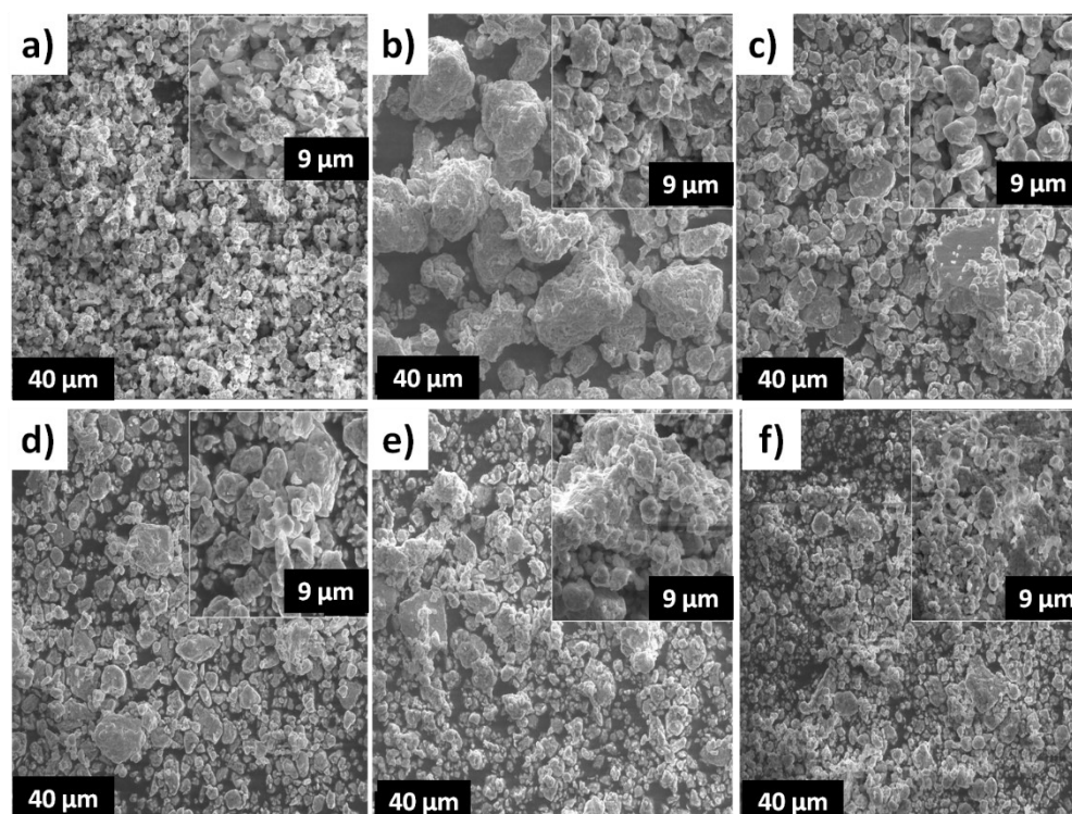
Figure 1. Scanning electron micrographs (SEM) of mechanically milled powders: (a) 0 h, (b) 5 h, (c) 25 h, (d) 50 h, (e) 100 h and (f) 150 h.
