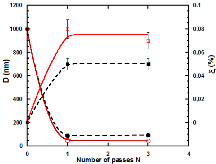
Figure 6: Crystallite size D (circles) and rms strain \xi (squares) of the as cast Al-7wt%Si alloy after ECAE at temperatures 20°C (open marks) and 160°C (full marks).
