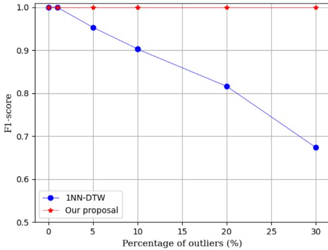
FIGURE 14 Sensitivity to outliers in the reference (training) database of the proposal compared to 1NN-DTW (benchmark)
