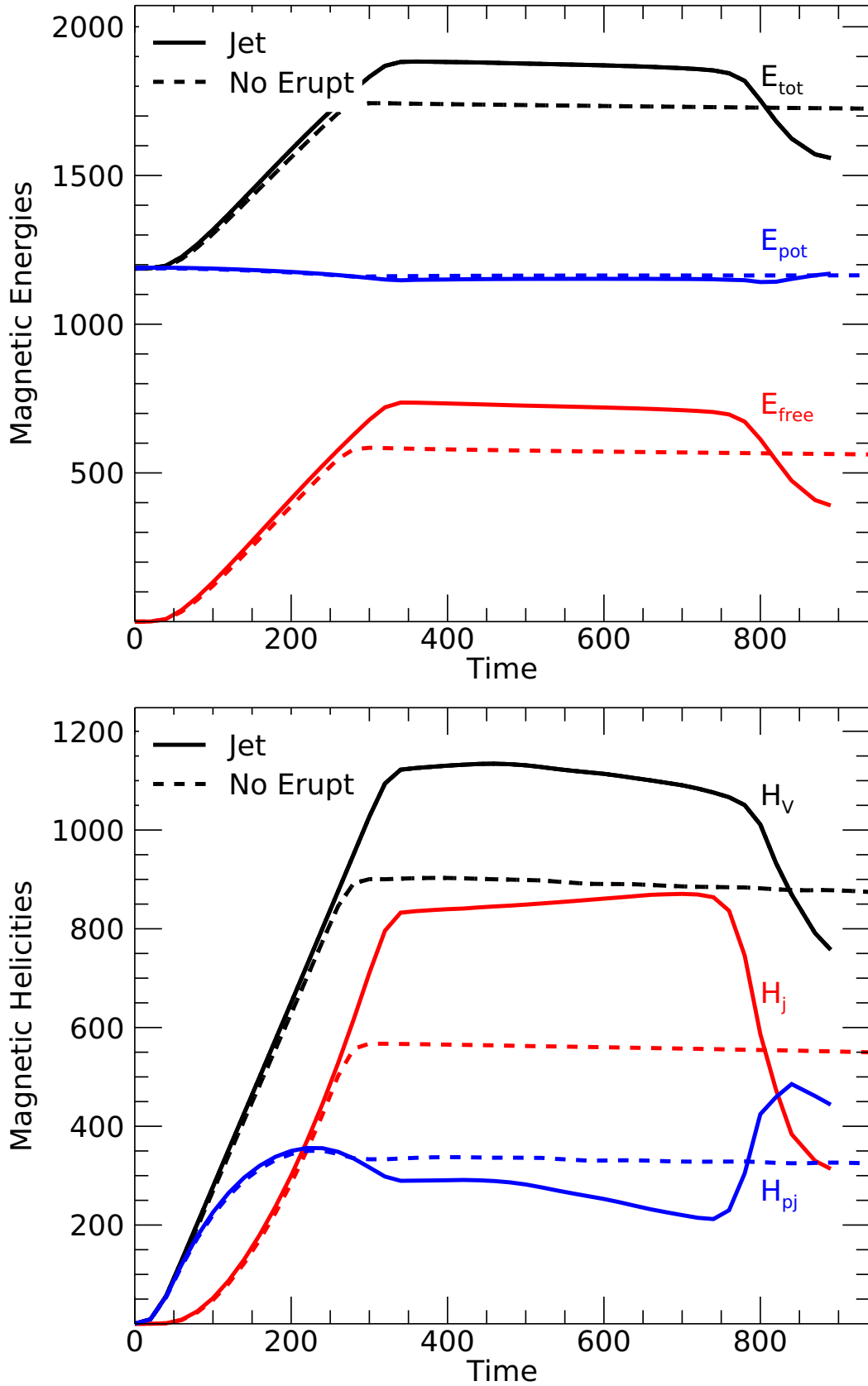
Fig. 4. Time evolution of the magnetic energies and helicities. Top panel: evolution of the total magnetic energy ( E_{\text{tot}} , black lines), potential magnetic energy ( E_{\text{pot}} , blue lines), and free magnetic energy ( E_{\text{free}} , red lines) in the non-eruptive (dashed lines) and in the jet-producing (continuous lines) simulations. Bottom panel: evolution of the total relative magnetic helicity ( H_V , black lines), non-potential magnetic helicity ( H_J , red lines), and volume-threading magnetic helicity ( H_{\text{pj}} , blue lines), in the non-eruptive (dashed lines) and in the jet-producing (continuous lines) simulations.
