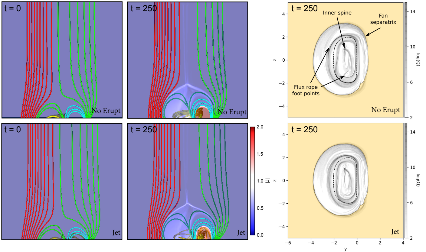
Fig. 1. Snapshots of the common initial phase ( 0 < t < 250 ) of both simulations. Left panels: electric current density distribution in a central 2D cut and magnetic field lines. Right: QSL distribution at t = 250 . The dashed line shows the PIL. Top panels: non-eruptive case. Bottom panels: jet-producing case. Yellow shading indicates the open field.
