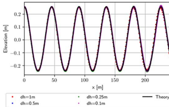
Figure 1. Mesh convergence study for wave propagation.
