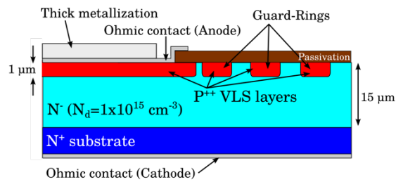
Fig. 2. Cross section of the fabricated diodes.
