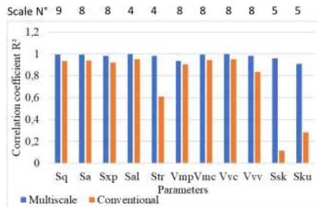
Figure. 10. Correlation coefficient for each parameter with wavelet decomposition and conventional approach
