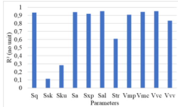
Figure 9. Correlation coefficient for each parameter
