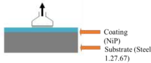
Figure. 3. Crash coating test schematic [8]
