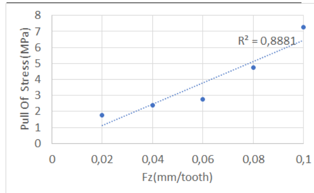
Figure. 4. Pull of stress evolution with F_z
