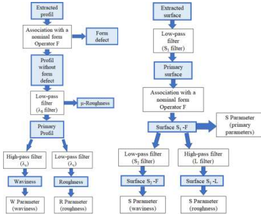
Figure. 1. a) Steps for a profile study ISO 4287-4288 profil procedure . b) Steps for an areal study ISO 25178 analysis procedure
