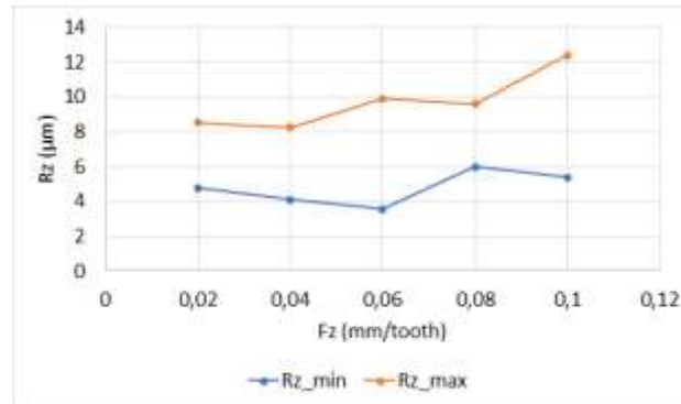
Figure. 5. Rz evolution with Fz
