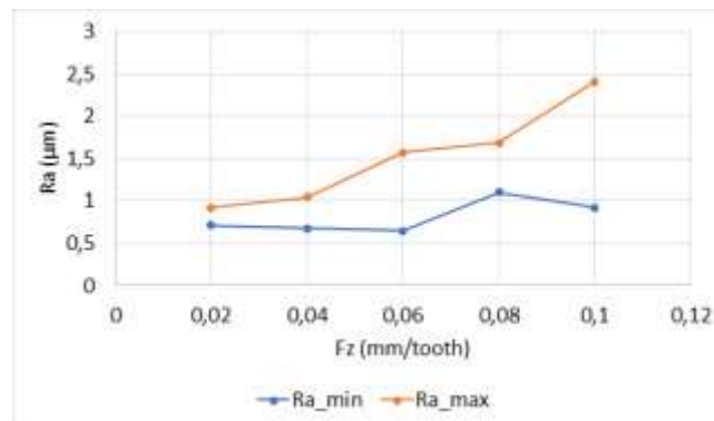
Figure. 6. Ra evolution with Fz
