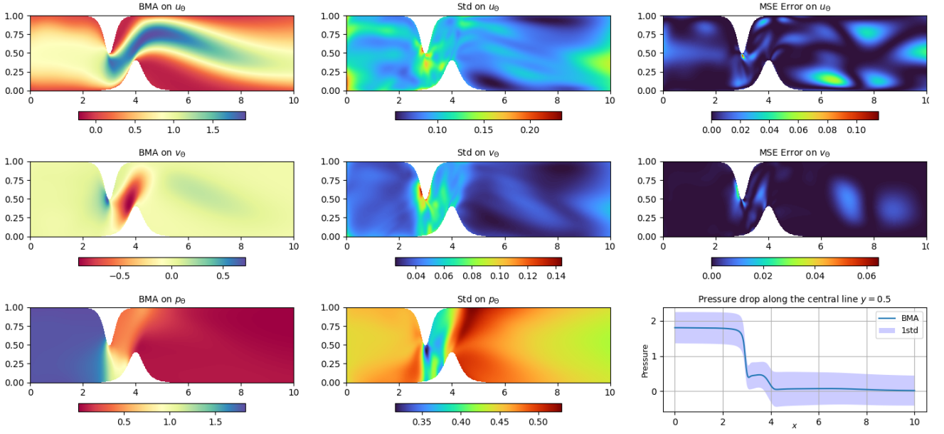
Figure 12: CFD inverse problem: BMA predictions of the velocity field \mathbf{u}_\theta = (u_\theta, v_\theta) in asymmetric stenosis along with their uncertainty standard deviations (Std) and mean squared errors (MSE), at the top. BMA and uncertainty on the inferred latent pressure field with the pressure evolution plotted along the central line y = 0.5 , leading to an average pressure drop of 1.78 — bottom.
