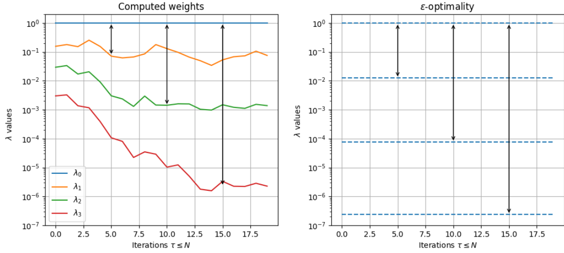
Figure 6: Evolution of the \lambda_k weights along the adaptive steps ( \tau \leq N ) on the left, and comparison with analytical \varepsilon -optimal weights for Sobolev training up to third-order derivative. Evolution of Average weights over several repetitions of the AW-HMC algorithm. This is induced by different initializations of the neural network parameters and momentum, to take into account sample variability. The order of magnitude of the relative weights \lambda_0/\lambda_i , i = 1 \dots 3 are represented by the double-headed arrows.
