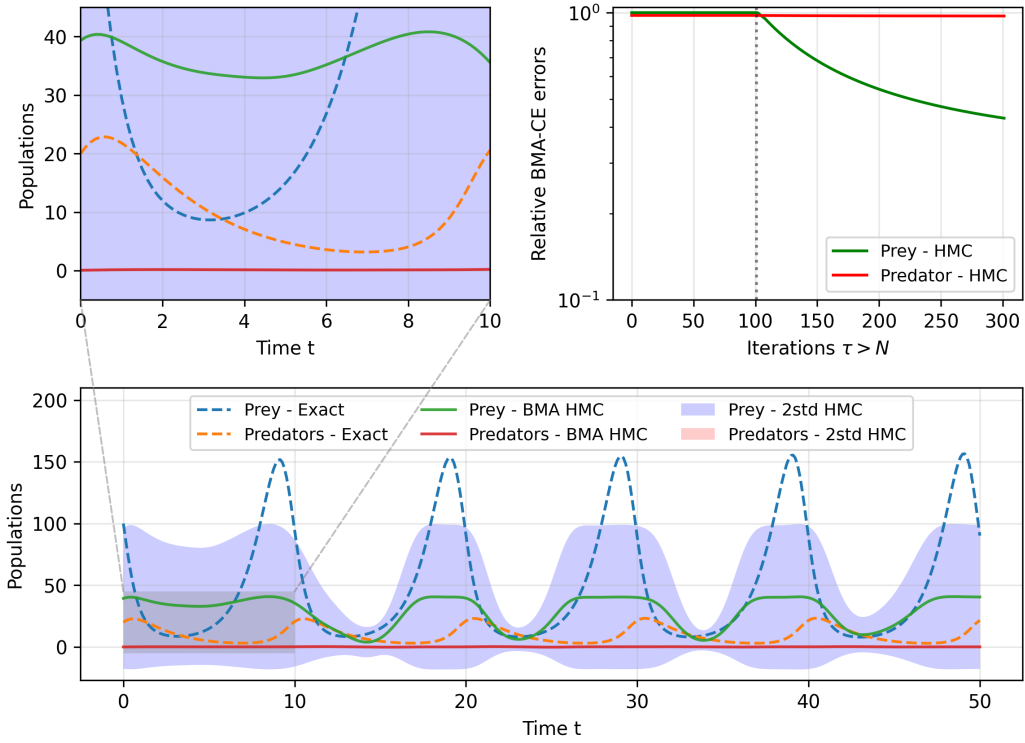
Figure 17: Failure mode of classical HMC, with uniform weighting, on the Lokta-Volterra multi-scale inverse problem defined in Sect. 3.3. BMA predictions for the two-species populations along the physical time with their uncertainties — bottom and top left figures. Relative BMA-CE errors throughout the sampling iterations illustrate lack of convergence of the method — top right.
