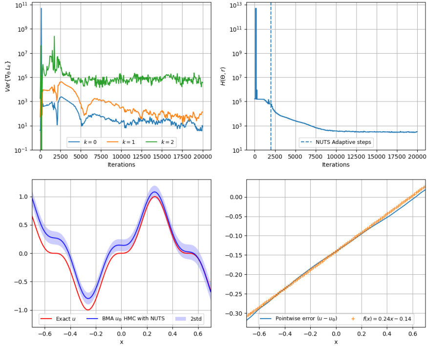
Figure 2: Failure mode of NUTS step-size adaptation in Sobolev training up to second order derivatives: variances of the effective gradient \nabla_{\Theta} L_k distributions (top left) and Hamiltonian evolution (top right), respectively showing task imbalances and weak exploration of the energy levels. Signal approximation (bottom left) and pointwise error (bottom right) highlighting the linear deviation of u_{\Theta} . The vertical dotted line delimits the number of adaptive steps in the NUTS sampler.
