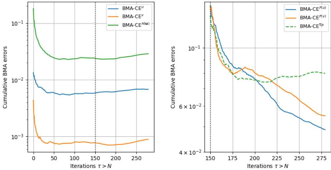
Figure 13: CFD inverse problem: Bayesian Model Average Cumulative Errors throughout the sampling iterations for the velocity field components \mathbf{u} = (u, v) , the divergence-free condition \mathcal{H}(\mathbf{u}) , on the left, and the PDE residuals \mathcal{F}(u) and \mathcal{F}(v) , on the right. The dotted curve represents the a posteriori checking of pressure gradient norm BMA-CE error as defined in equation (40)
