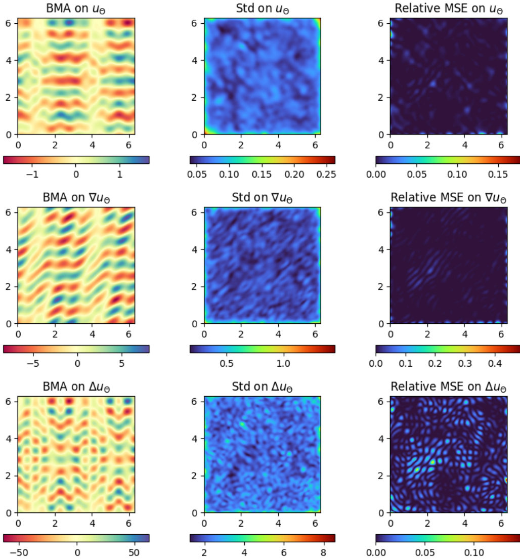
Figure 16: 2D Sobolev training benchmark: BMA predictions, predicted standard deviation, and relative BMA errors, presented locally for each term of the multi-objective potential energy. We worked on a limited case l = 8 with about 15% of training points. The global relative BMA errors, averaged over the entire domain, scale around 1.69e - 3 , 3.42e - 3 , and 5.6e - 3 respectively.
