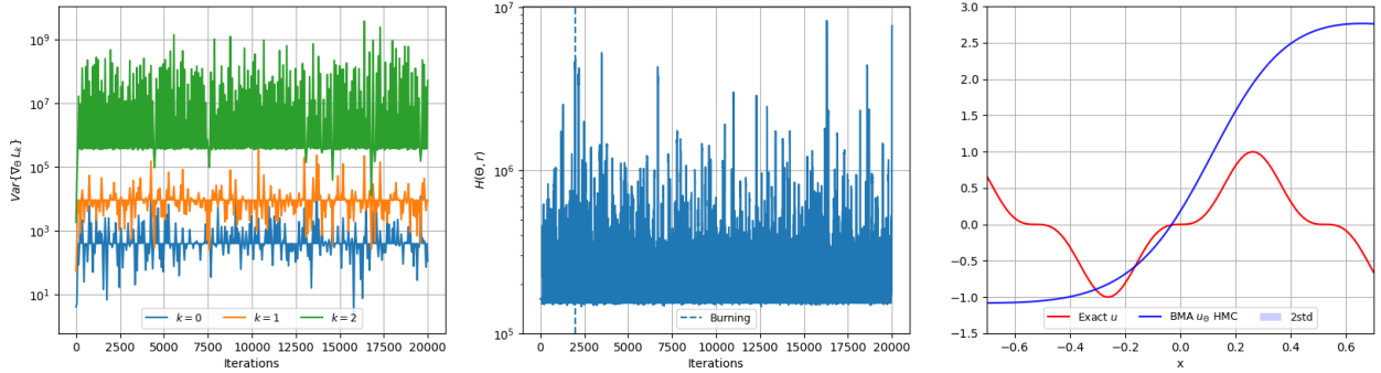
Figure 1: The HMC uniform-weighting failure mode for Sobolev training up to second-order derivatives leading to non-conservative Hamiltonian (on the middle), and extremely poor resulting approximation of the function (on the right). This is due to the strong imbalances in the variances of the effective gradient \nabla_{\Theta} L_k distributions ( k = 0, 1, 2 ), plotted with respect to the (N_s \times L) HMC iterations (on the left).
