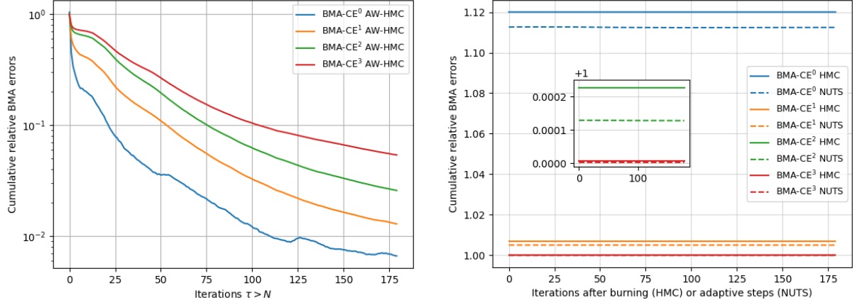
Figure 7: Cumulative relative BMA errors, computed according to equation (28), throughout the sampling iterations \tau > N for Sobolev training up to third-order derivative. Comparison between the AW-HMC strategy (on the left) and classical HMC and NUTS formulations (on the right). These quantities remain nearly constant in pathological cases, due either to massive rejection or pathological random walk, highlighting the lack of convergence in the usual BPINNs-HMC formulations (on the right).
