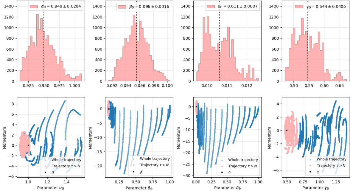
Figure 8: Lotka-Volterra multi-scale inference: histogram of the marginal posterior distributions for the inverse parameters \alpha_\theta , \beta_\theta , \delta_\theta and \gamma_\theta (top). Phase diagrams of the parameter trajectories throughout the sampling (bottom) that characterized convergence toward their respective modes during the adaptive steps (in blue) and efficient exploration of the mode neighborhood after the adaptive steps (in red). The ground truth parameters are respectively \alpha = 1 , \beta = 0.1 , \delta = 0.01 and \gamma = 0.5 and establish an inverse problem with separate scales.
