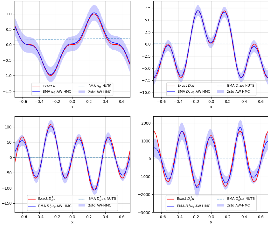
Figure 5: 1D Sobolev training up to third-order derivative: comparison of the BMA predictions, on the function and its derivatives, between the AW-HMC and NUTS formulations. The imbalance between tasks and random walk behavior of NUTS (see Fig 4) results in ineffective BMA predictions. The AW-HMC methodology overcomes these effects and significantly improves the sampling of the target distribution.
