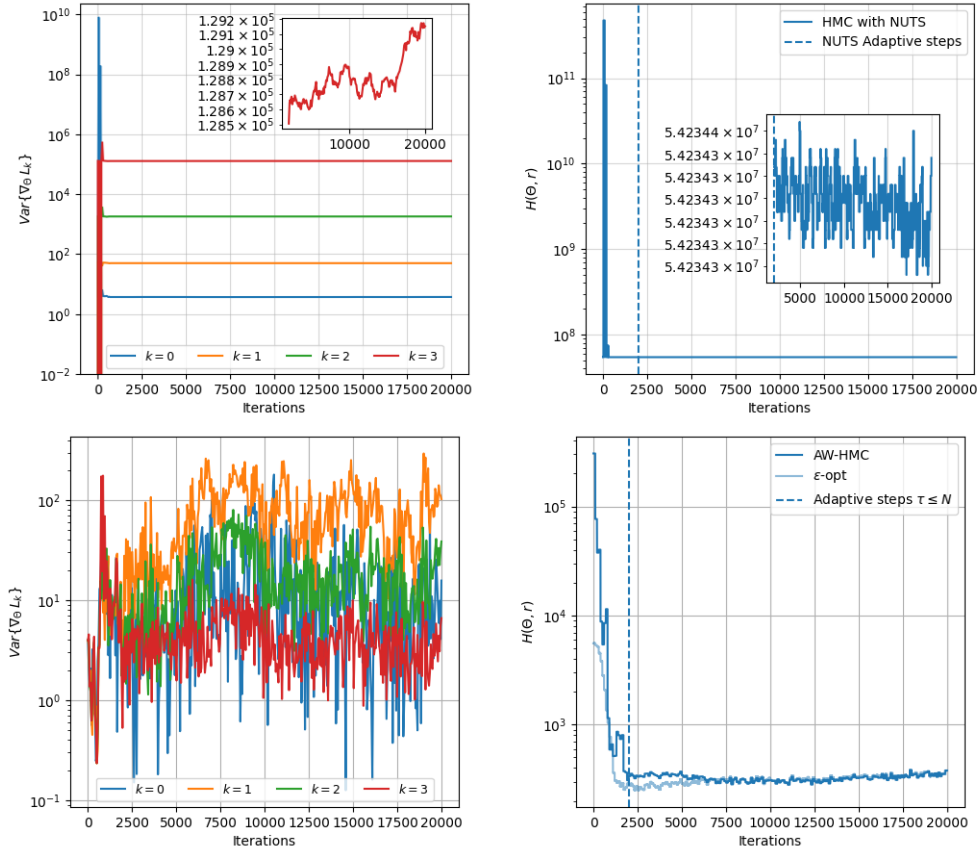
Figure 4: Effective gradient distribution variances \text{Var}\{\nabla_{\Theta} L_k\} and Hamiltonian evolution on 1D Sobolev training up to the third-order derivative. The NUTS formulation (top) highlights strong imbalances between the learned tasks, on the left, and random-walk behaviors in exploring the energy level sets, on the right. AW-HMC strategy (bottom) and comparison with the \epsilon -optimality.
