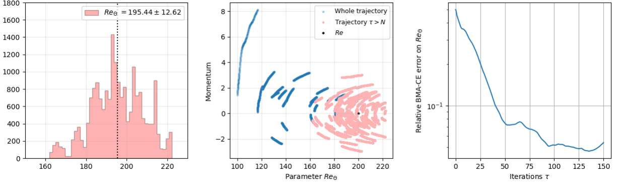
Figure 14: CFD inverse problem: from left to right, histogram of the marginal posterior distribution for the inverse Reynolds parameter, phase diagram of its trajectory throughout the sampling and BMA-CE error using the absolute relative norm as defined in (39). The relative BMA-CE error on Re_\Theta is plotted over the all the \tau iterations of the second step sampling in the sequential training.
