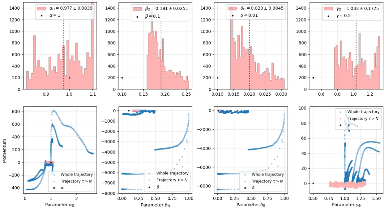
Figure 19: Failure mode of HMC with NUTS on the Lotka-Volterra multi-scale inference: histogram of the marginal posterior distributions for the inverse parameters (top) and phase diagrams of their trajectories throughout the sampling (bottom). The biased predictions from Fig 18 prevent proper inference of the inverse parameters, leading to random walk pathological behavior in the updated parameters.
