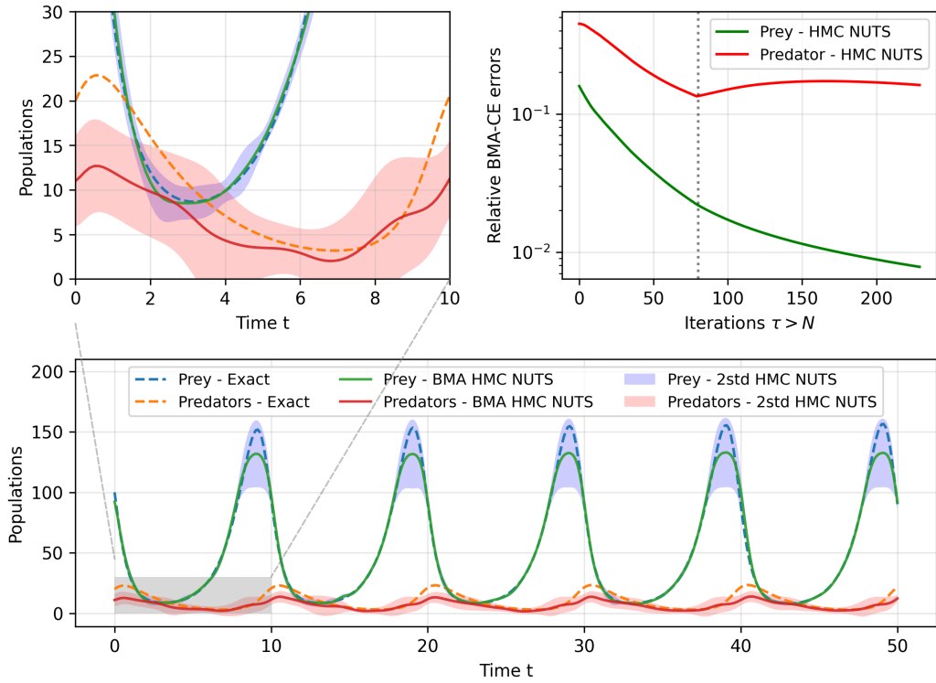
Figure 18: Failure mode of HMC with NUTS adaptation on the Lotka-Volterra multi-scale inverse problem defined in Sect. 3.3. BMA predictions for the two-species populations along the physical time with their uncertainties — bottom and top left figures. Relative BMA-CE errors throughout the sampling iterations showing an imbalance between the tasks and preferential adaptation of the prey population — top right figure.
