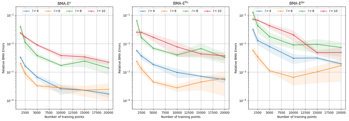
Figure 15: 2D Sobolev training benchmark: comparison of the relative BMA errors, as defined in (27), plotted with respect to the number of training points for various shape complexities induced by the different values of l . The number of training points is increased until about 30% of the whole data set is reached, for 20000 training points.
