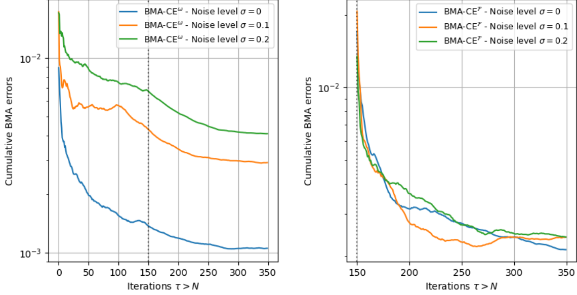
Figure 10: Vorticity physics-informed inpainting problem: Bayesian Model Average Cumulative Error diagnostics, as defined in (35), throughout the sampling iterations and for different noise levels. BMA-CE on the vorticity field prediction (on the left) and on the PDE residual \mathcal{F} satisfying (33) (on the right). The dotted vertical lines mark the introduction of the PDE constraint in sequential training.
