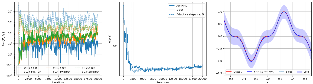
Figure 3: Adaptively Weighted Hamiltonian Monte Carlo (AW-HMC) on Sobolev training up to second-order derivatives compared to \varepsilon -optimal weighting. Effective gradient distributions variances \text{Var}\{\nabla_{\Theta} L_k\} with balanced conditions between the tasks (on the left). Hamiltonian evolution throughout the sampling satisfying energy conservation (in the middle). Resulting field predictions with a comparison between \varepsilon -optimal results and AW-HMC strategy (on the right).
