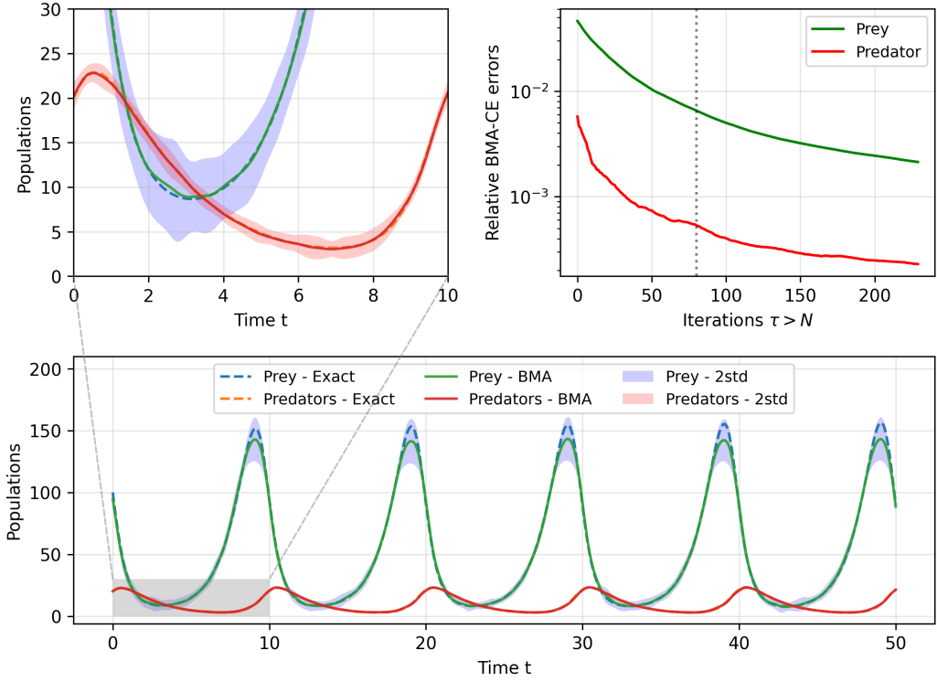
Figure 9: Lokta-Volterra multi-scale inference: BMA predictions of the two-species populations along the physical time with their uncertainties, bottom and top left. Relative BMA-CE errors defined as in equation (28) for the neural network outputs y = (u_\Theta, v_\Theta) plotted throughout the sampling iterations, — top right. The dotted vertical line marks the introduction of the ODE-likelihood terms in the sequential training.
