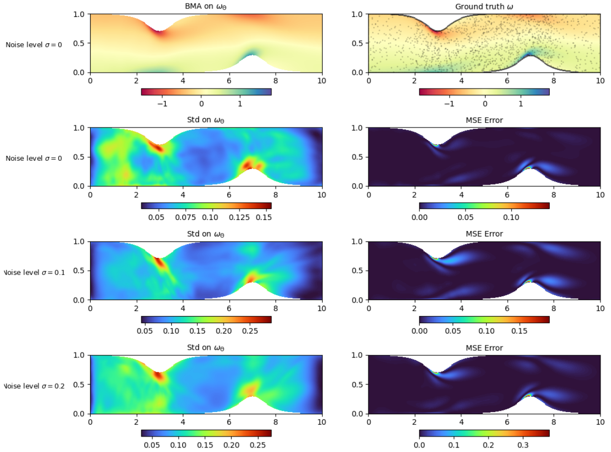
Figure 11: Physics-informed inpainting problem: BMA prediction of the vorticity field \omega_\Theta in asymmetric stenosis without noise, compared to the ground truth solution \omega (top). The black dots on the exact field correspond to the training measurements of the dataset \mathcal{D} . Comparison of the uncertainty standard deviations (Std) and mean squared errors (MSE) on the predicted vorticity field \omega_\Theta for different noise levels ( \sigma = 0, 0.1, 0.2 ), shown in the bottom rows.
