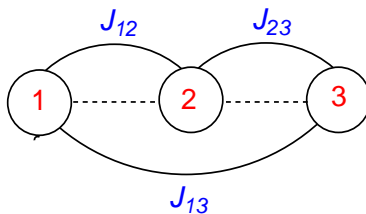
Scheme 3: different exchange coupling interactions
