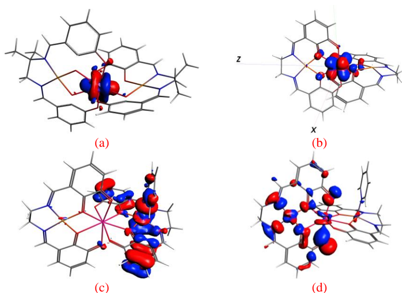
Figure 5: Iso-surfaces density maps of the (a) SOMO, (b) SOMO-1, (c) SOMO-24 and (d) SOMO-25 or the L^1CuUCuL^1pyr complex (isodensity surface at 0.0025 \text{ e bohr}^{-3} )
