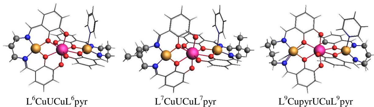
Figure 1: Representation of the optimized molecular structures of the L^iCuUCuL^i complexes. Pink, yellow, red and blue balls are used for emphasizing uranium, copper, oxygen and nitrogen atoms, respectively.
