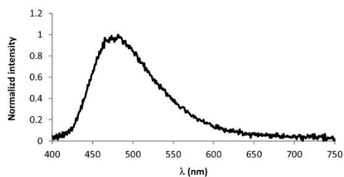
Figure 4. Emission spectra pseudo-para disubstituted pCp 15 at the solid state ( \lambda_{\text{ex}} = 360 nm, \lambda_{\text{em}} = 480 nm).
