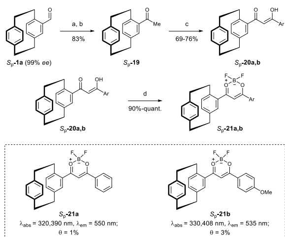
Scheme 7. Representative synthesis of an enantiopure pCp-based boron- \beta -diketonate ( S_p - 18 ). Both enantiomers were prepared following this strategy. Reaction conditions: (a) MeMgBr (1.3 equiv.), THF, 0 °C to rt, 1.5 h; (b) DMP (1.5 equiv.), CH 2 Cl 2 , rt, 2 h; (c) ArCO 2 Me (2 equiv.), NaH (5 equiv.), THF, 75 °C, 24 h; (d) BF 3 ·Et 2 O (1.9 equiv.), toluene, rt or 120 °C, 18 h. Spectroscopic data were recorded in CH 2 Cl 2 (10 -6 M solutions). Relative fluorescence quantum yields were determined using anthracene as the reference ( \theta = 2.6\% in cyclohexane).
