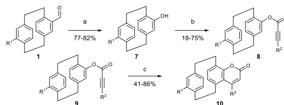
Scheme 4. Synthesis of pCp-based coumarins. Reaction conditions: (a) H 2 O 2 (1.4 equiv.), H 2 SO 4 (1.4 equiv.), CH 2 Cl 2 /MeOH, rt, overnight; (b) Propiolic acid derivative (1 equiv.), DCC (1 M in CH 2 Cl 2 , 1.5 equiv.), DMAP (0.015 equiv.), CH 2 Cl 2 , Ar, rt, 2-4 h; (c) AuCl 3 (0.08 equiv.), AgSbF 6 (0.16 equiv.), \mu\text{w} , DCE, Ar, 80 °C, 7 min.
