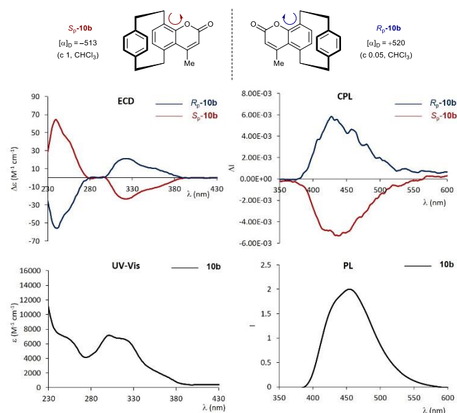
Figure 2. Chiroptical properties of pCp-based coumarins S P -10b and R P -10b . UV-Vis, PL, ECD and CPL spectra were recorded in CH 2 Cl 2 (10 -5 M solutions, \lambda_{\text{ex}} = 320 nm).
