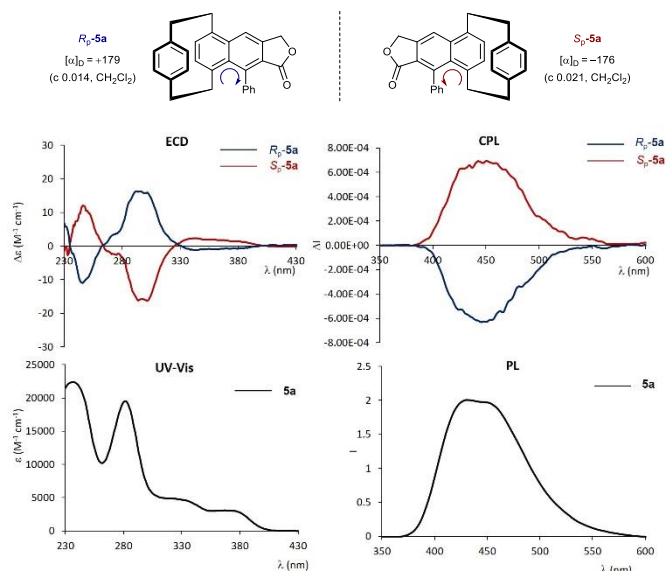
Figure 1. Chiroptical properties of pCp-based naphthalenes S p -5a and R p -5a. UV-Vis, PL, ECD and CPL spectra were recorded in CH 2 Cl 2 (10 -5 M solutions, \lambda_{\text{ex}} = 365 \text{ nm} ).
