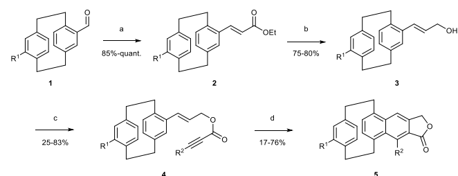
Scheme 3. Synthesis of pCp-based naphthalenes. Reaction conditions: (a) Triethyl phosphonoacetate (1.5 equiv.), DBU, Ar, rt, 4 h; (b) DIBAL-H (4 equiv.), Et 2 O, Ar, –78 °C to rt, 4 h; (c) Propiolic acid derivative (1.05 equiv.), DCC (1 M in CH 2 Cl 2 , 1.5 equiv.), DMAP (0.01 equiv.), CH 2 Cl 2 , Ar, rt, 4 h; (d) \mu w, PhNO 2 , 180 °C, 30 min.
