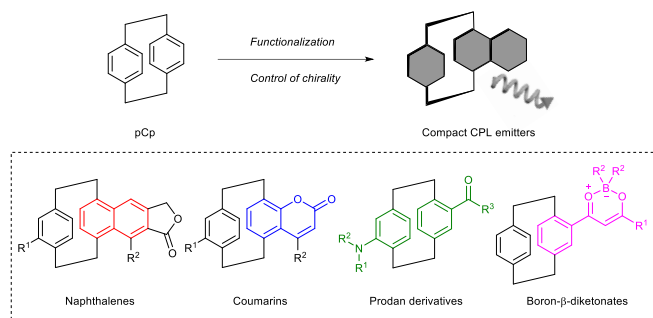
Scheme 1. Different families of compact CPL emitters based on the pCp scaffold.
