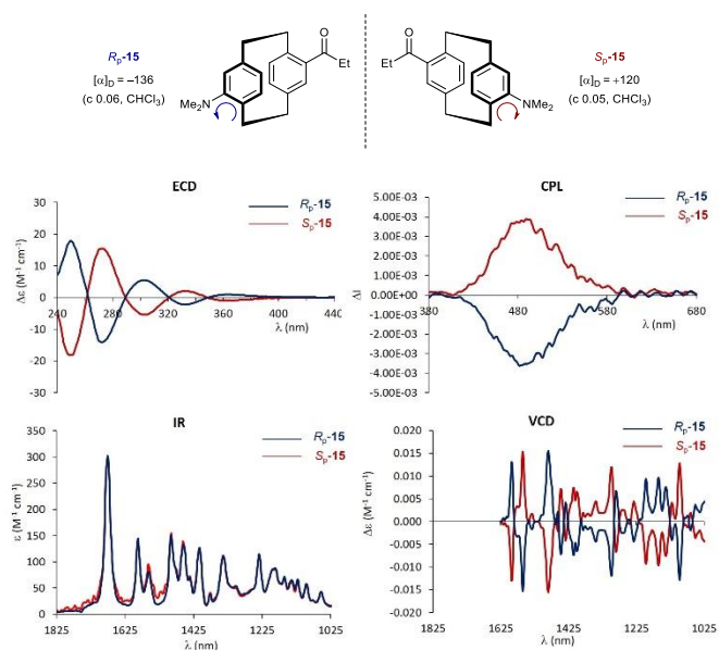
Figure 5. Chiroptical properties of pCp-based PRODAN analogues R_p - 15 and S_p - 15 . ECD spectra were recorded in toluene (10 -3 M solutions). CPL spectra were recorded in toluene (10 -5 M solutions). IR and VCD spectra were recorded in CD 2 Cl 2 (10 -1 M solutions, 200 microns pathlength).
