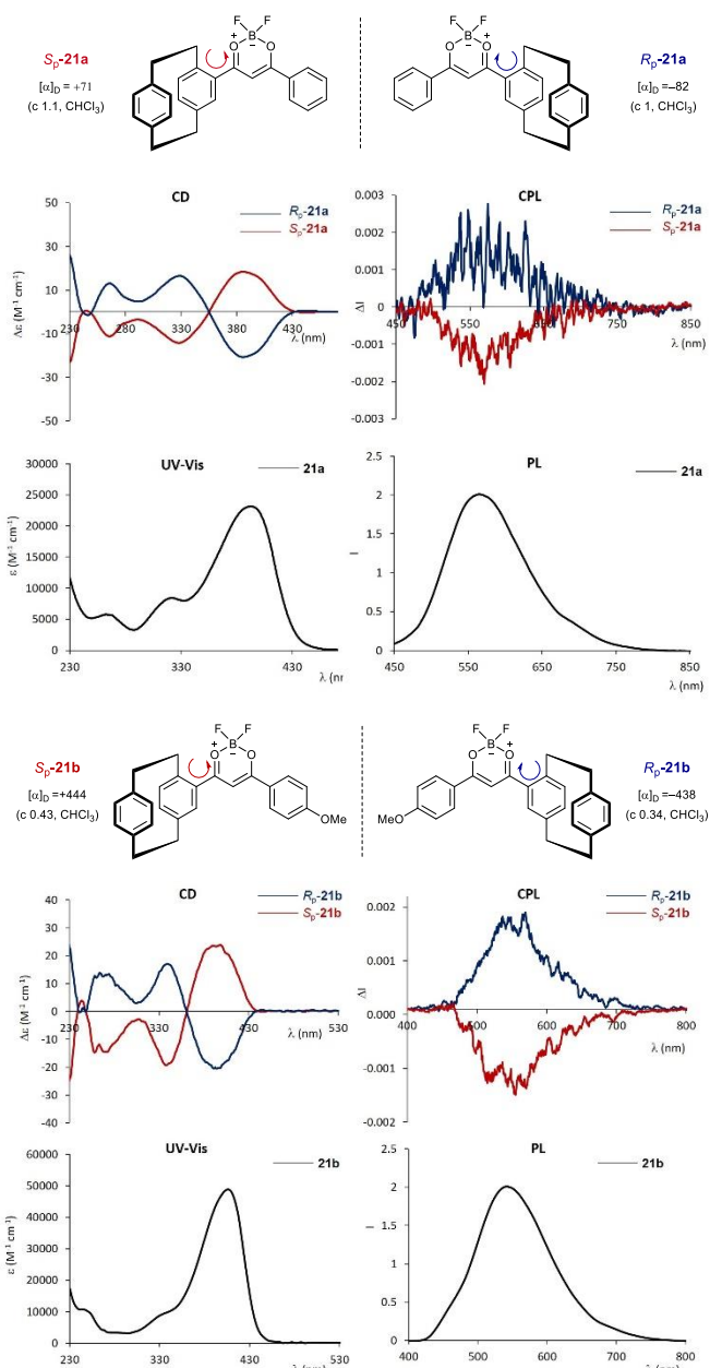
Figure 6. Chiroptical properties of pCp based \beta -diketonates R_p - 21a,b and S_p - 21a,b . UV-Vis and ECD spectra were recorded in CH 2 Cl 2 (10 -4 M solutions). PL and CPL spectra were recorded in CH 2 Cl 2 (10 -5 M solutions, \lambda_{\text{exc}} = 360 \text{ nm} ).
