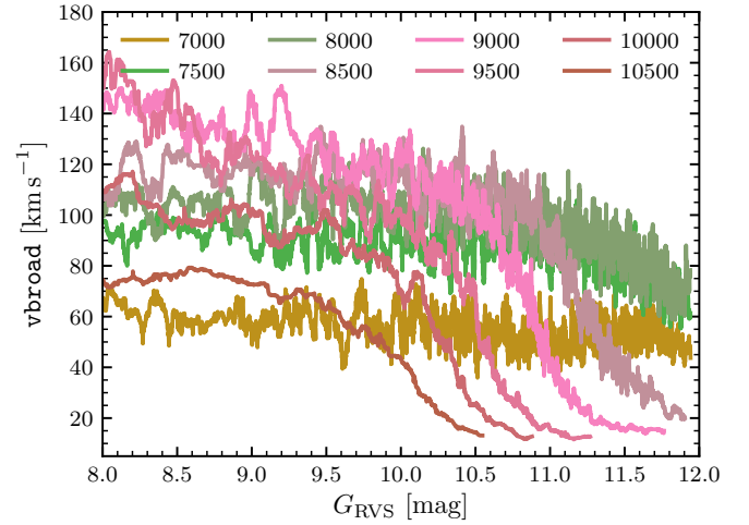
Fig. 14. Median value of vbroad as a function G_{RVS} for different T_{\text{eff}} . Temperatures are taken as exact rv_template_teff values, and median vbroad are derived on a running window of 200 points. Each colour corresponds to a T_{\text{eff}} labelled in the plot.
