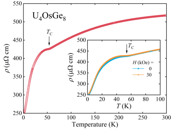
Figure 6 Temperature dependence of electrical resistivity \rho of U_4OsGe_8 . Inset: \rho(T) below 100 K measured in various magnetic fields.
