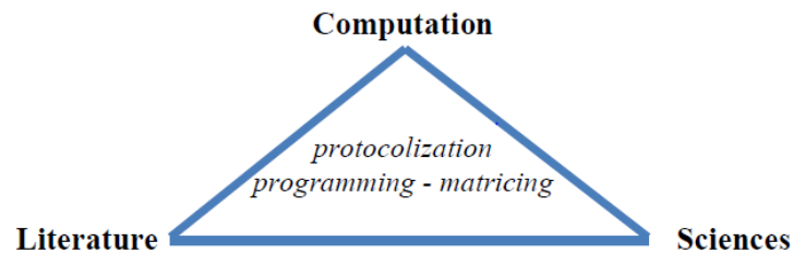
Figure 1: First diagram of triangulation.
