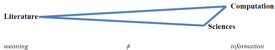
Figure 2: Second diagram of triangulation.
