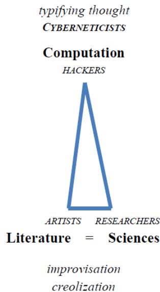
Figure 3: Third diagram of triangulation.
