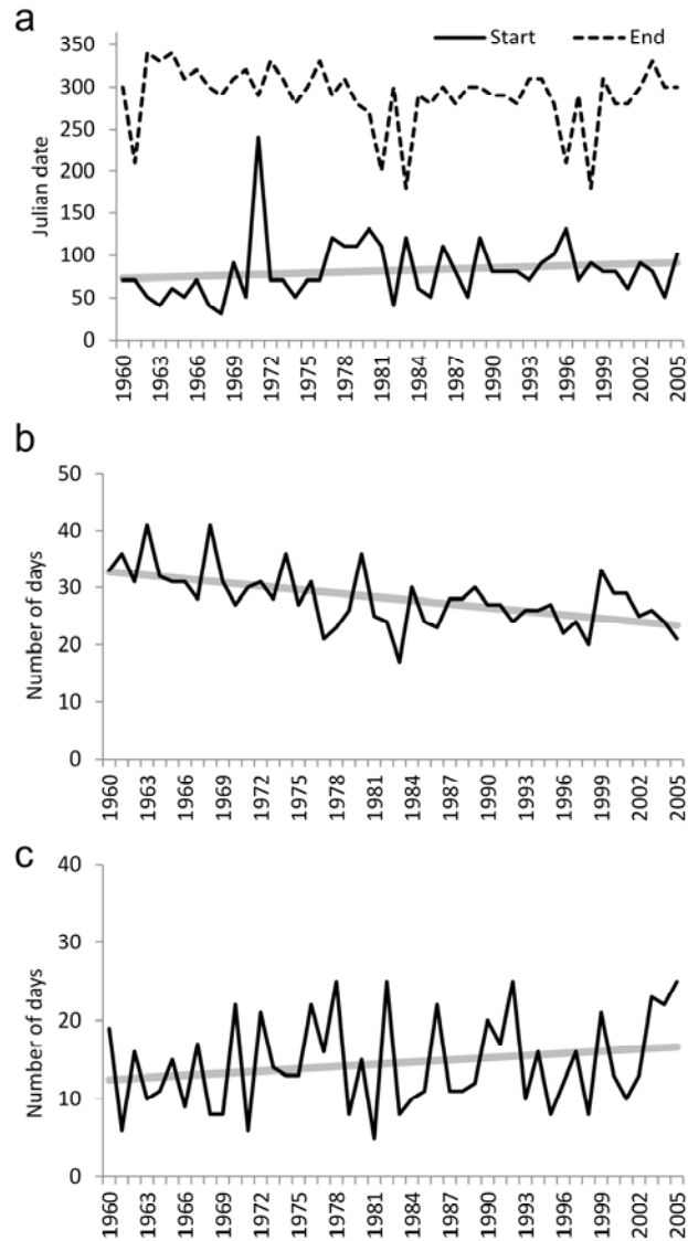
Figure 5. Time series for variables 25 and 26 (a), variable 27 (b) and variable 28 (c) at Kumasi station. Grey lines: significant trends at 95% confidence level
