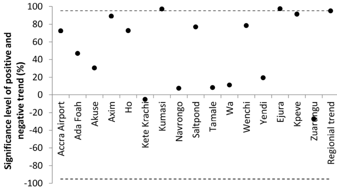
Figure 7. Significance level of trends observed for variable 28 (length of the longest wet season rainless period). Positive and negative values correspond to positive and negative trends, respectively. Dotted lines: 95% significance level
