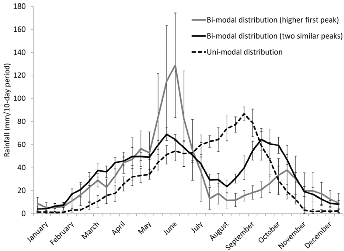
Figure 2. Seasonal rainfall patterns in Ghana, derived from 16 studied rainfall stations, averaged over period (1960-2005). Grey solid curves: average from stations Axim, Ada Foah, Accra Airport, Saltpond. Black solid curve: average from stations Akuse, Ho, Kumasi, Wenchi, Ejura, Kpeve. Dotted curve: average from stations Kete Krachi, Navrongo, Tamale, Wa, Yendi, Zuarungu. Vertical error bars: standard deviation between stations
