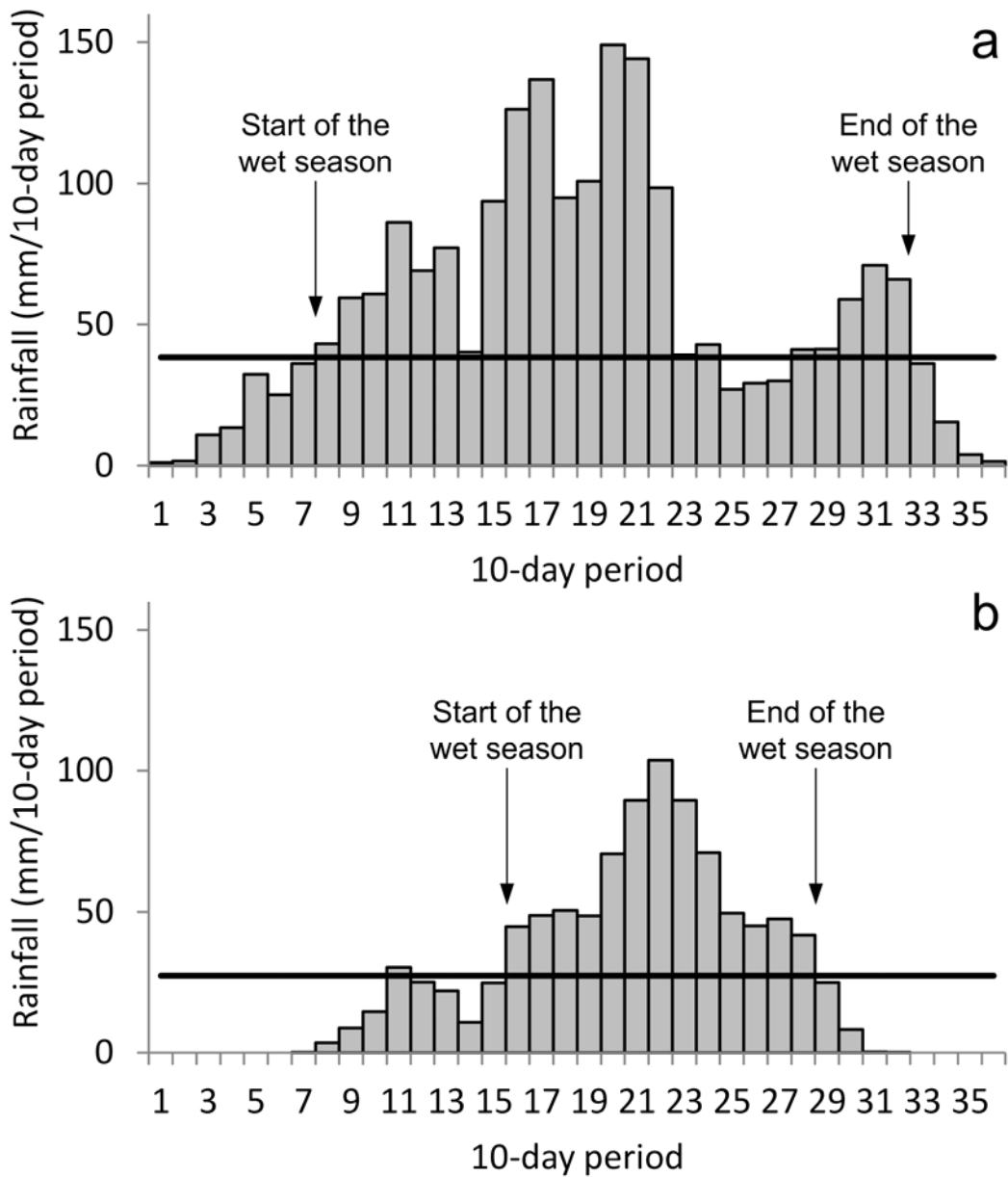
Figure 3. Graphical illustration of method used to determine the start (variable 25) and end (variable 26) of the wet season at Kumasi (a) and Navrongo (b) for example year 1966. Horizontal line: mean 10-day rainfall depth averaged over period 1960-2005.
