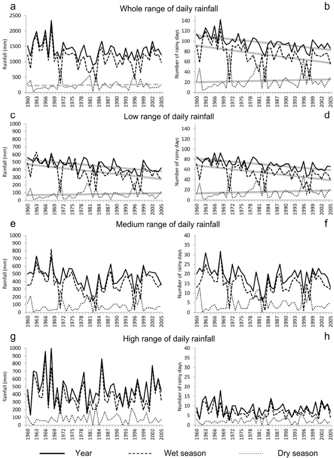
Figure 4. Time series for variables 1 to 12 (a, c, e, g) and variables 13 to 24 (b, d, f, h) at Kumasi station. Solid and dotted grey lines: significant trends at 95% and 90% confidence levels, respectively
