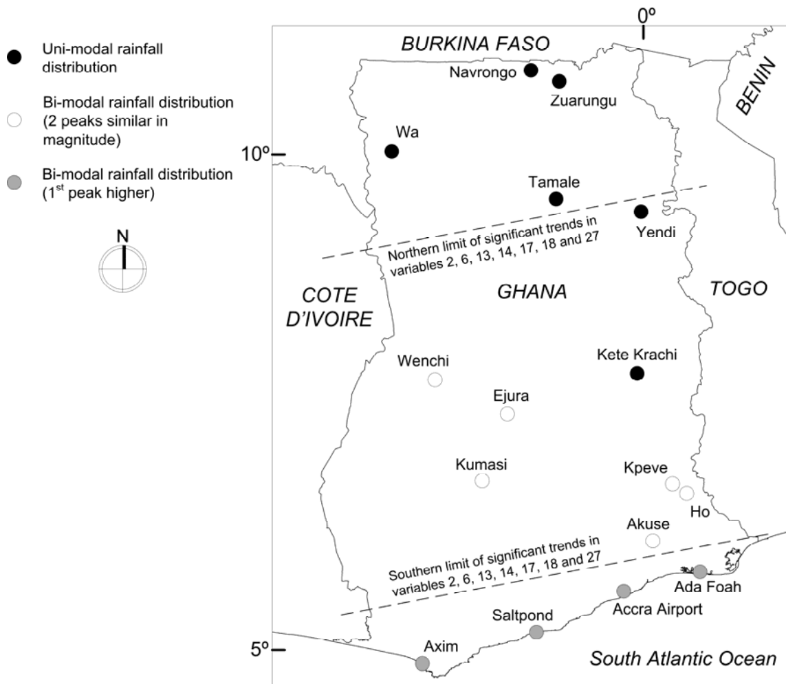
Figure 1. Location of rainfall stations, types of rainfall pattern and areas exhibiting negative trends in rainfall depths and number of rainy days as presented in Table 2 and Figure 2
