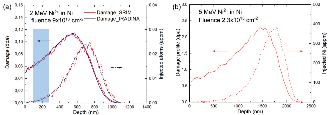
Fig. A. 1 Damage profile of (a) 2 MeV \text{Ni}^{2+} ions injected into Ni by SRIM 2013 code and IRADINA code for a fluence of 9 \times 10^{13} ions. \text{cm}^{-2} ; and (b) 5 MeV \text{Ni}^{2+} ions injected into Ni for a fluence of 2.3 \times 10^{15} ions. \text{cm}^{-2} The displacement threshold energy of Ni is taken as 40 eV [3,57]
