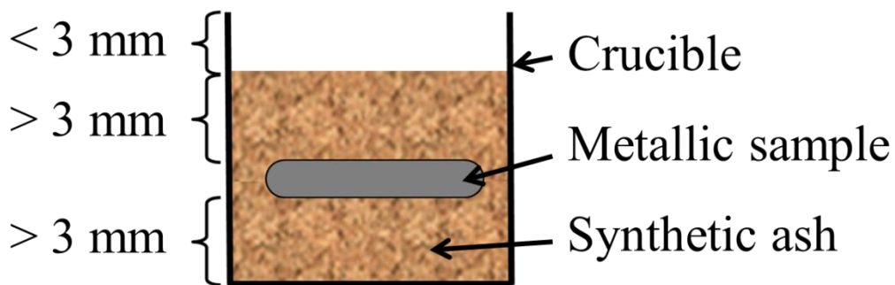
Fig. 1 Scheme of corrosion test settings
