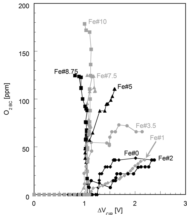
Fig. 11—Delay and background-corrected oxygen levels (O 2 BC) vs the corrected cell voltage V CIR ; temperature: 1824 K ± 3, Ar-gas flow: 0.05 STP m 3 h -1 , scanning rate 0.17 mV s -1 .
