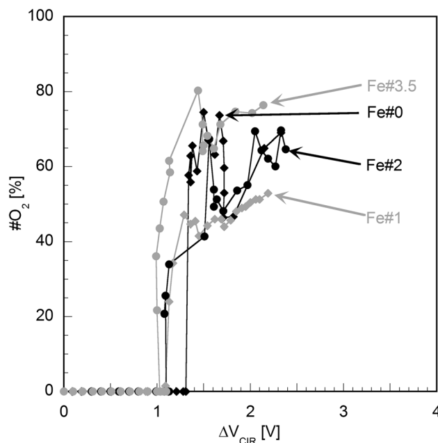
Fig. 12—Anodic yield in the compositions Fe#0, Fe#1, Fe#2 and Fe#3.5 in dependence of the cell voltage; temperature: 1824 K ± 3, Ar-gas flow: 0.05 STP m 3 h -1 , scanning rate 0.17 mV s -1 .
