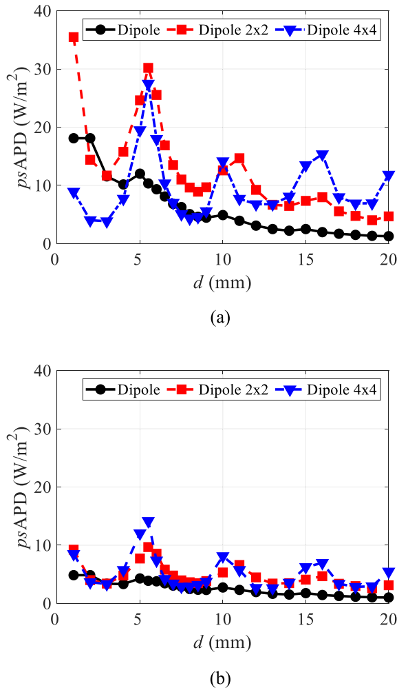
FIGURE 11. sAPD as a function of antenna-to-skin separation distance with different antenna types of single dipole, 2 \times 2 , and 4 \times 4 dipole arrays at 30 GHz averaged over (a) 1 \text{ cm}^2 and (b) 4 \text{ cm}^2 .
