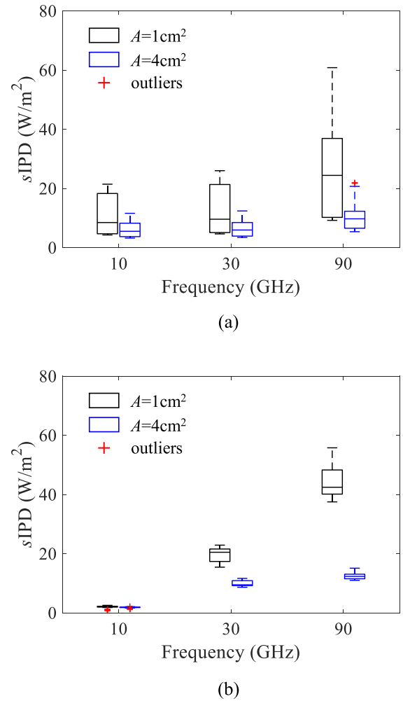
FIGURE 8. Statistical analysis of sIPD as a function of frequency from 10 to 90 GHz considering all the potential effects caused by the EM-method, antenna-to-skin separation distance, definition of power density, and averaging area: (a) single dipole and (b) 4 \times 4 dipole arrays.
