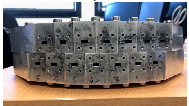
FIGURE 11. Manufactured prototype: (a) View from the array of septum polarizers, (b) View from the input ports.
