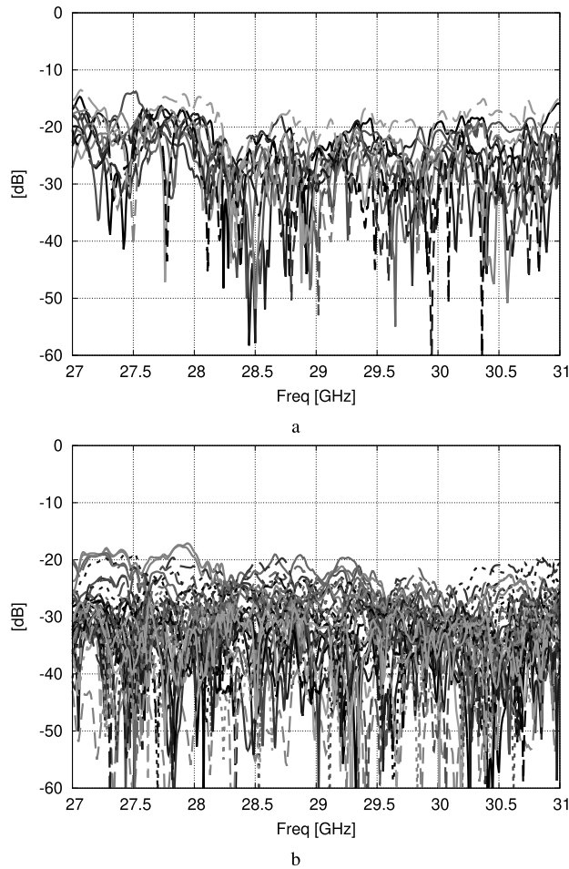
FIGURE 12. Scattering parameters (S-matrix) of the measured prototype: (a) Reflection coefficient for each input port, (b) Mutual coupling between the feeding ports.
