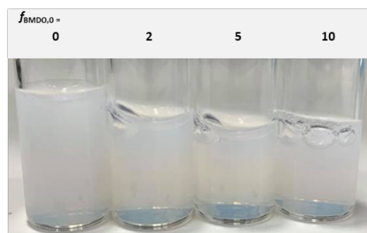
Figure 4. Photos of the latexes prepared with different initial molar fraction of BMDO. From left to right: experiments E1MMA, f_{\text{BMDO},0} = 0\% ; E4BMDO, f_{\text{BMDO},0} = 2\% ; E1BMDO, f_{\text{BMDO},0} = 5\% ; E5BMDO, f_{\text{BMDO},0} = 10\% (Table 1).
