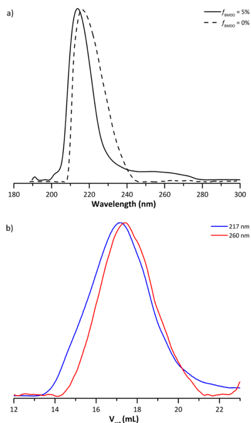
Figure 3 a) SEC traces from the UV detector obtained for the dried extract from experiments E1MMA ( f_{\text{BMDO},0} = 0\% ) and E1BMDO ( f_{\text{BMDO},0} = 5\% , Table 1), normalized on the maximum of absorption. b) SEC traces from the UV detector set at 217 nm (blue) and 260 nm (red) obtained for experiment E1BMDO (Table 1).
