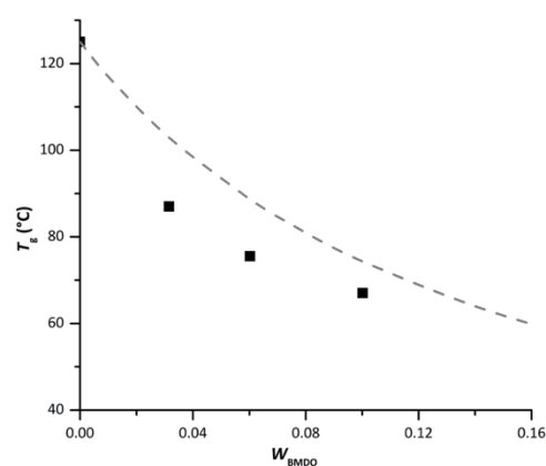
Figure 7. Evolution of experimental (square) and theoretical (dashed line) T_g with the mass fraction of BMDO. Theoretical values were calculated with the Fox equation.
