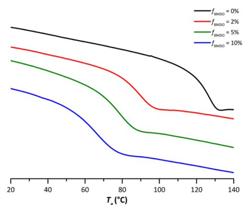
Figure 6. Thermograms from DSC analyses performed on the dried extract of latexes of PMMA (E1MMA) and P(MMA-co-BMDO) with increasing amounts of BMDO: f_{\text{BMDO},0} = 2\% (E4BMDO), f_{\text{BMDO},0} = 5\% (E1BMDO), f_{\text{BMDO},0} = 10\% (E5BMDO) (Table 1).
