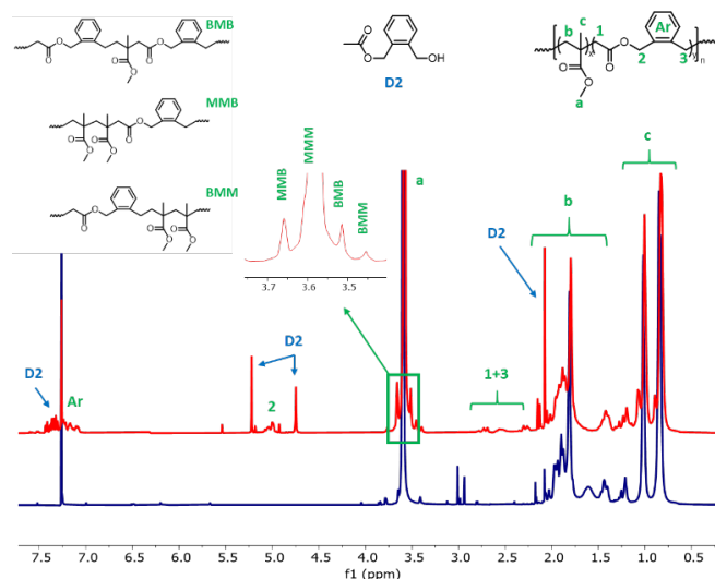
Figure 2. ^1\text{H} NMR spectra of the dried extract of latexes E1BMDO (red) and E1MMA (blue) ( \text{CDCl}_3 , 256 scans). Assignments were made according to a previous report. 13 B stands for BMDO units and M for MMA units in a triad. D2 corresponds to one of the identified degradation products of BMDO (D2 - see supporting information, Figure S1).
