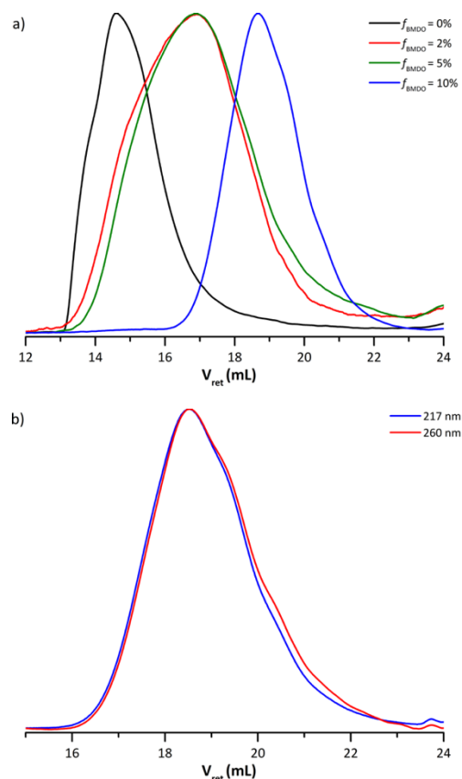
Figure 5. a): Molar mass distributions of dry extracts for latexes E4BMDO (red), E5BMDO (blue), E1BMDO (green) and EMMA1 (black) (Table 1). b) UV chromatograms from SEC-THF analysis at 217 nm (blue) and 260 nm (red) for the dried latex E5BMDO.
