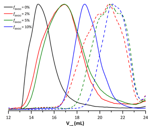
Figure 8. Molar mass distribution of dry extracts (plain lines) and degradation products (dashed lines) obtained by degradation of dry extracts using KOH in THF/MeOH for latexes synthesized with varying fraction of BMDO in the feed of monomers (black: E1MMA; red: E4BMDO; green: E1BMDO; blue: E5BMDO, Table 2).
