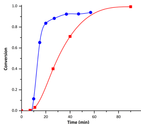
Figure 1. Evolution of MMA conversion with time during emulsion (co)polymerization of MMA and BMDO for experiments E1MMA (blue) and E1BMDO (red).
