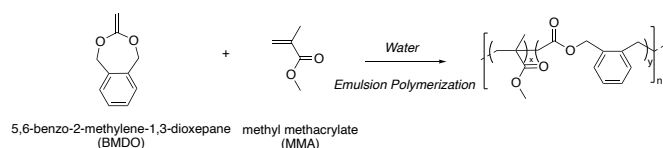
Scheme 1. Radical copolymerization of BMDO and MMA in aqueous emulsion polymerization.
