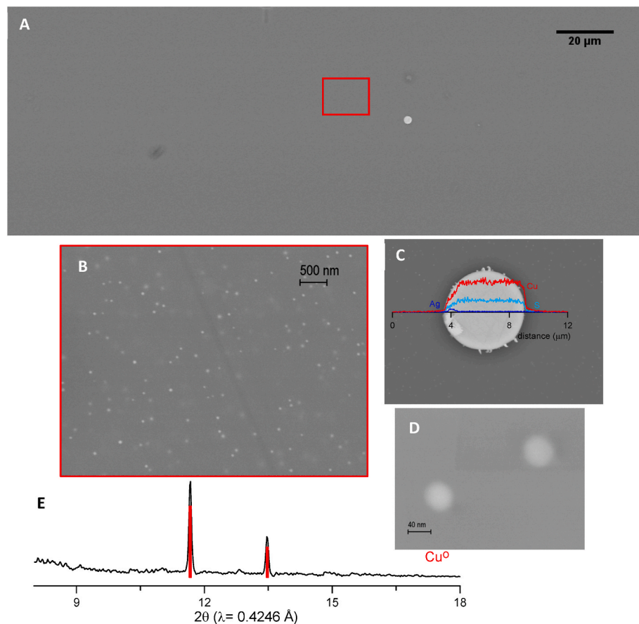
Fig. 4. (A) SEM-BSI image of a Medieval red glass SC13 (1284–1320, Monastery of Santes Creus, Tarragona) showing the presence of a micrometric Cu_2S particle (B) Magnification of the red square area from (A) showing the presence of small metallic copper nanoparticles. (C) Magnification and S, Cu and Ag linescan corresponding to one of the Cu_2S particles showing the presence of Ag_2S precipitated at the edge and (D) magnification of the metallic copper nanoparticles. (E) Micro-XRD pattern taken from a cross section of the red glass showing the presence of metallic copper, ICCD file 01-85-1326. (For interpretation of the references to colour in this figure legend, the reader is referred to the Web version of this article.)
