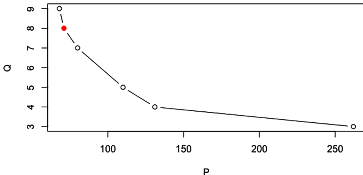
Figure 2: Pareto frontier with \rho -NF solution in red, \rho = 2
