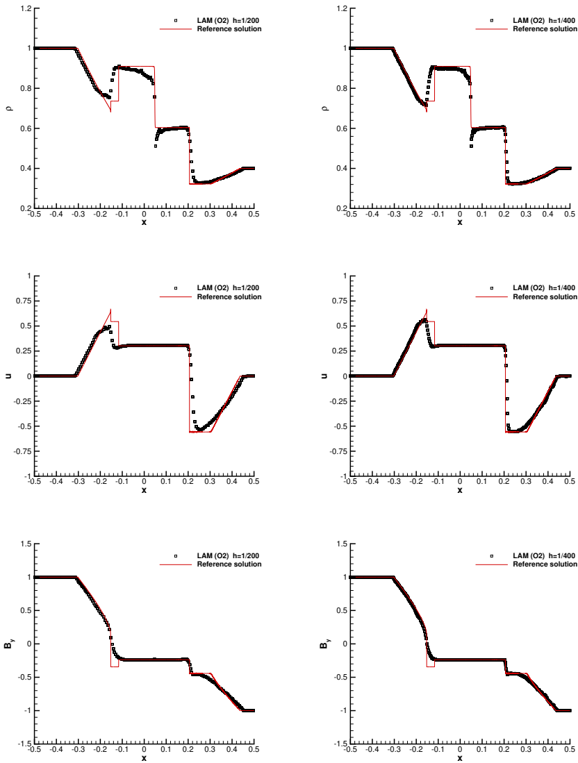
Fig. 9 MHD shock tube problem RPS8 at time t_f = 0.16 . Numerical solution for density (top), horizontal velocity (middle) and magnetic field component B_y (bottom) with characteristic mesh size h = 1/200 (left column) and h = 1/400 (right column row).
