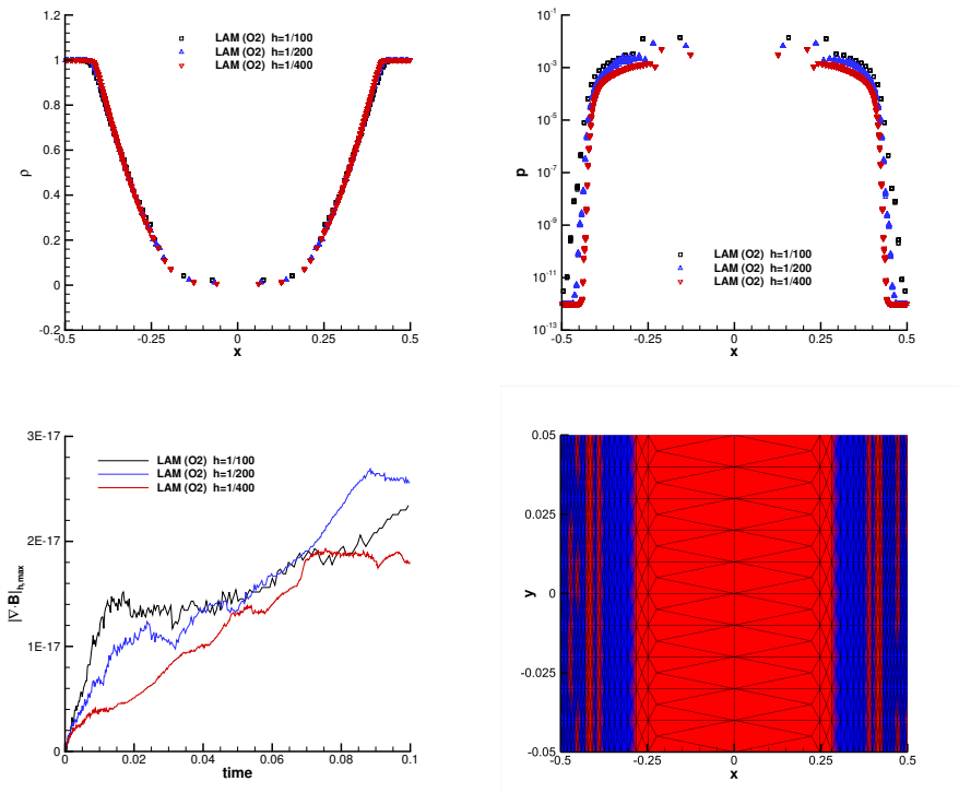
Fig. 11 MHD super-fast expansion test. Top: mesh convergence for second order solution for density (left) and pressure (right). Bottom: time evolution of the maximum value of |\nabla \cdot \mathbf{B}|_{h,\max} (left) and cell order map with mesh configuration for h = 1/100 (right).
