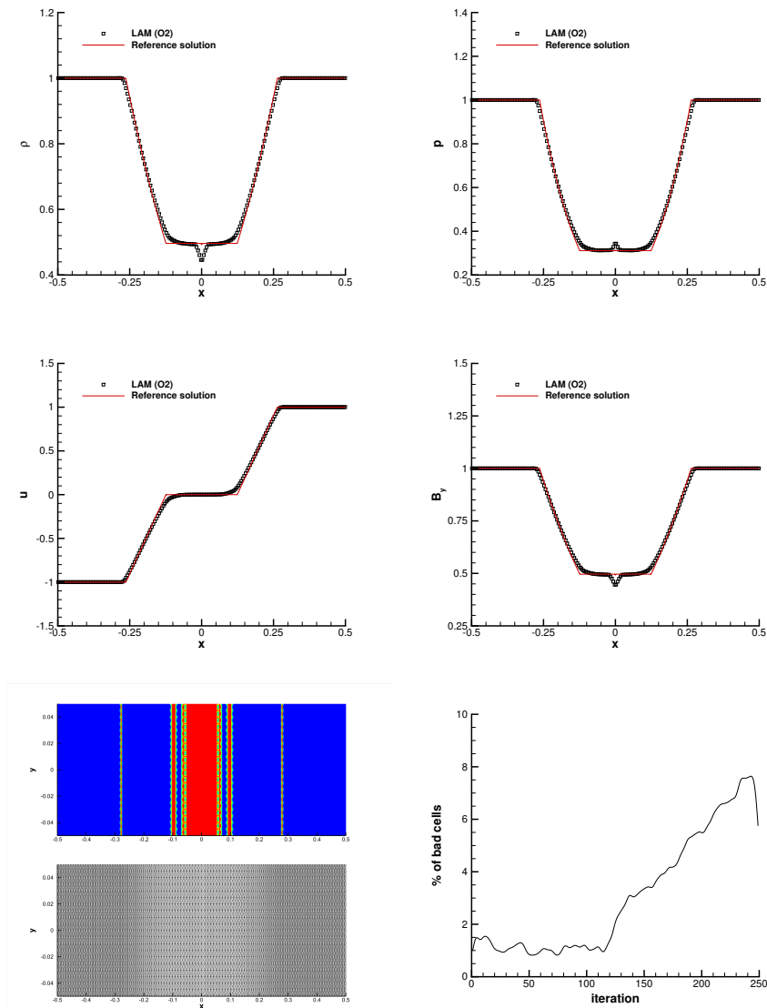
Fig. 5 MHD shock tube problem RP1 at time t_f = 0.1 . Numerical solution for density, pressure, horizontal velocity, magnetic field component B_y , cell order map with mesh configuration and percentage of detected bad cells at each iteration (from top left to bottom right).
