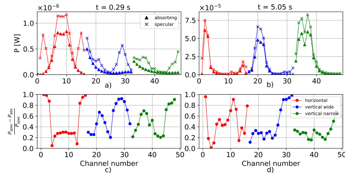
Figure 2. Simulated bolometer signals (a, b) for absorbing (triangles) and specular tungsten (crosses) models and their relative difference (c, d) for limiter (a, c) and flat-top (b, d) phases of the discharge
