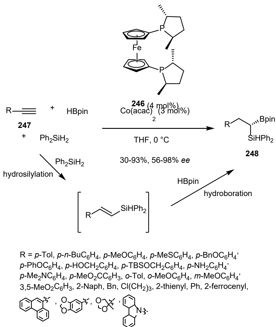
Scheme 63. Three-component domino hydrosilylation/hydroboration reaction of terminal alkynes, Ph 2 SiH 2 and HBpin in the presence of Me-Ferrocene ligand.
