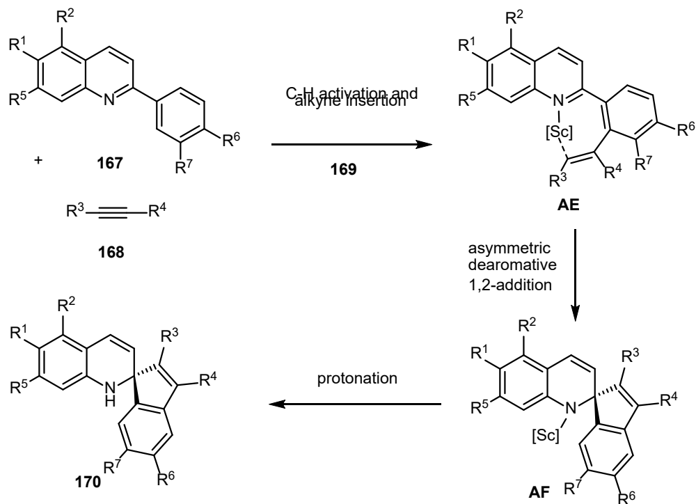
Scheme 42. Domino spiroannulation of 2-arylquinolines with alkynes.
