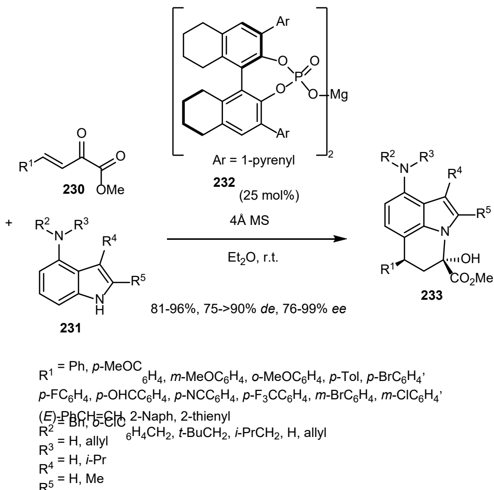
Scheme 59. Domino Friedel–Crafts alkylation/ N -hemiacetalization reaction of 4-aminoindoles with \beta,\gamma -unsaturated \alpha -ketoesters.
