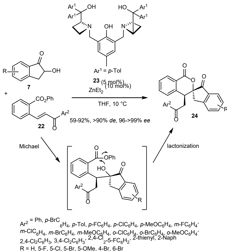
Scheme 7. Domino Michael/lactonization reaction of \alpha -hydroxy-1-indanones with ortho -ester chalcones.
