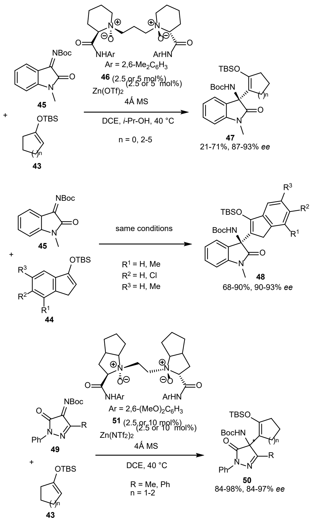
Scheme 12. Domino \alpha -alkenyl addition/proton shift reactions of silyl enol ethers with isatin- and pyrazolinone-derived ketimines.
