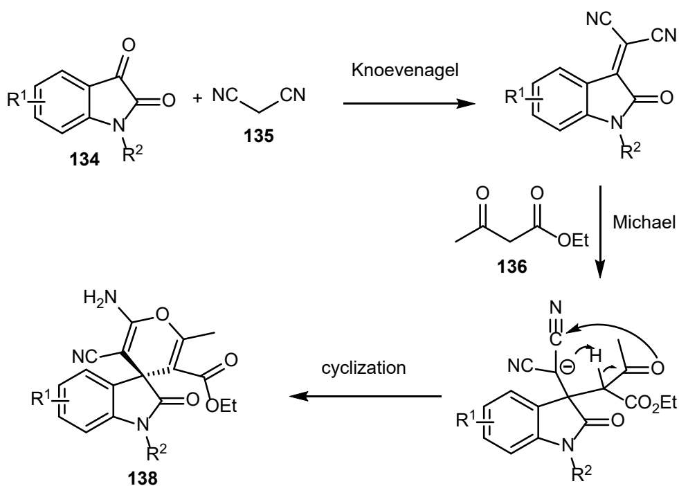
Scheme 35. Three-component domino Knoevenagel/Michael/cyclization reaction of isatins, malononitrile and ethyl acetoacetate.
