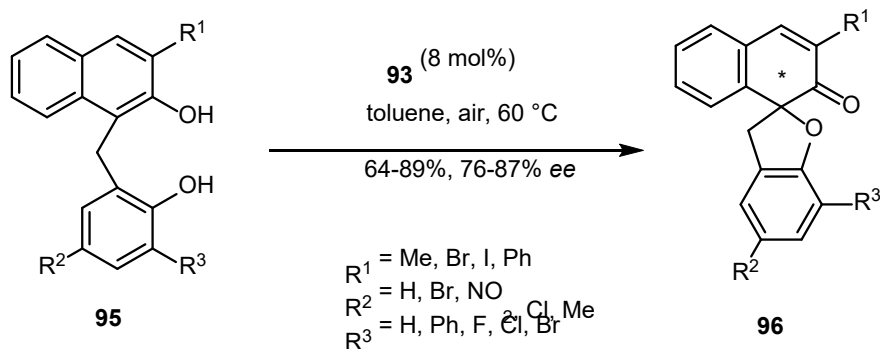
Scheme 24. Intermolecular and intramolecular domino dearomatization/spirocyclization reactions of 2-naphthols.
