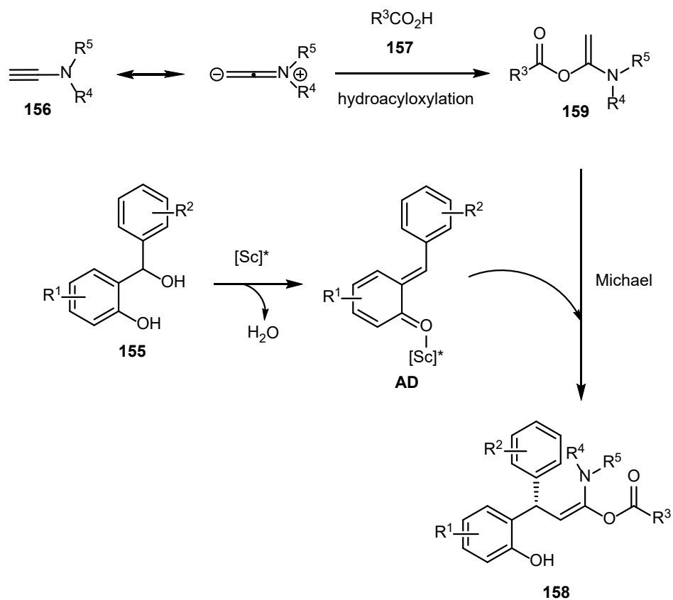
Scheme 40. Three-component domino hydroacyloxylation/Michael reaction of ortho -hydroxybenzyl alcohols, ynamides and carboxylic acids.
