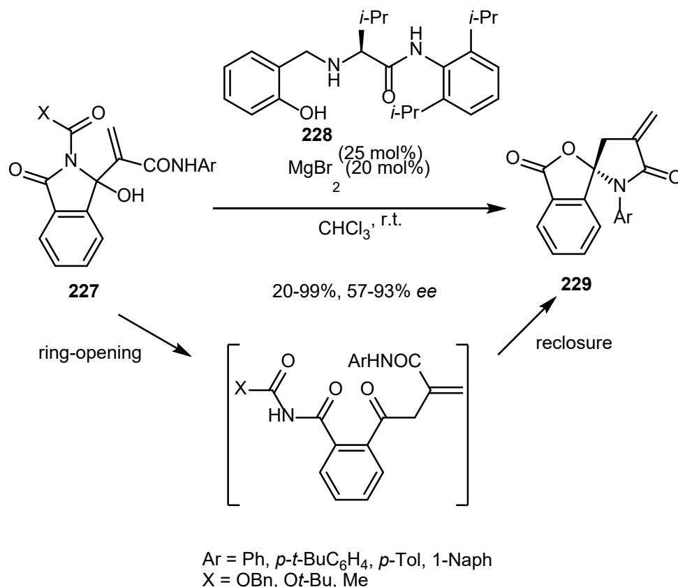
Scheme 58. Domino ring-opening/reclosure reaction of hydroxylactams.
