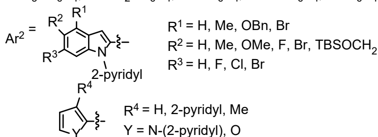
Scheme 62. Domino cyclization/C–H functionalization reaction of 1,6-enynes with indoles/pyrroles/furans.
