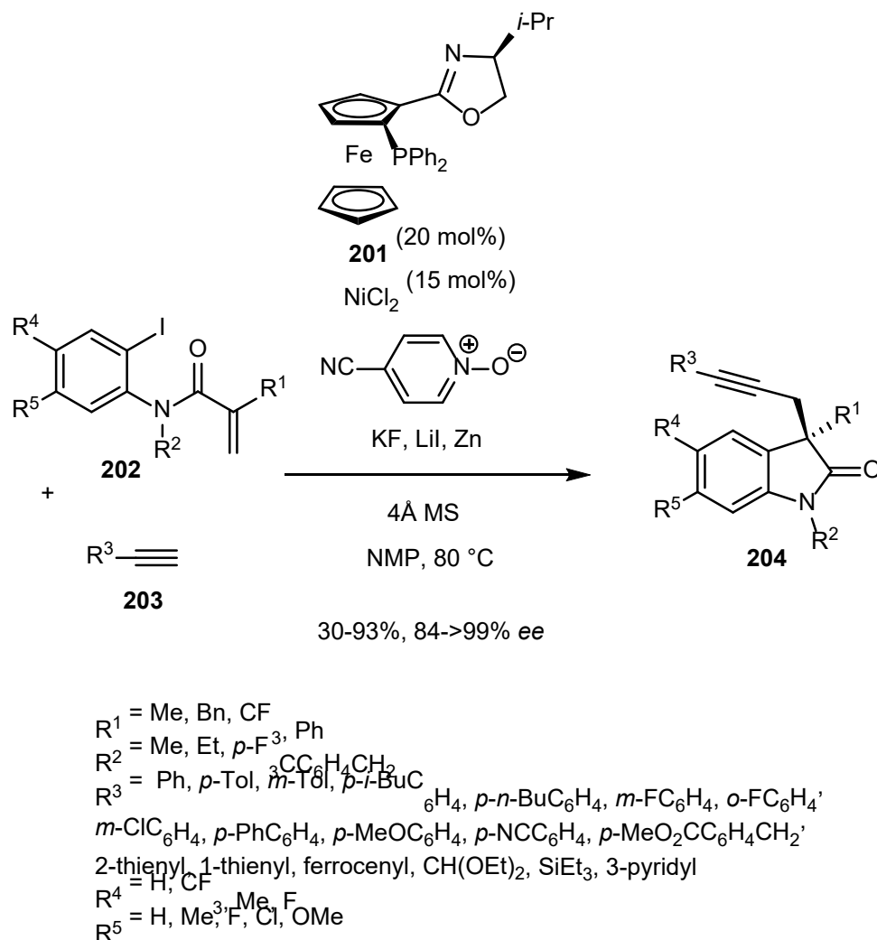
Scheme 51. Domino Heck/Sonogashira reaction of N -(2-iodophenyl)- N -alkylmethacrylamides with terminal alkynes.
