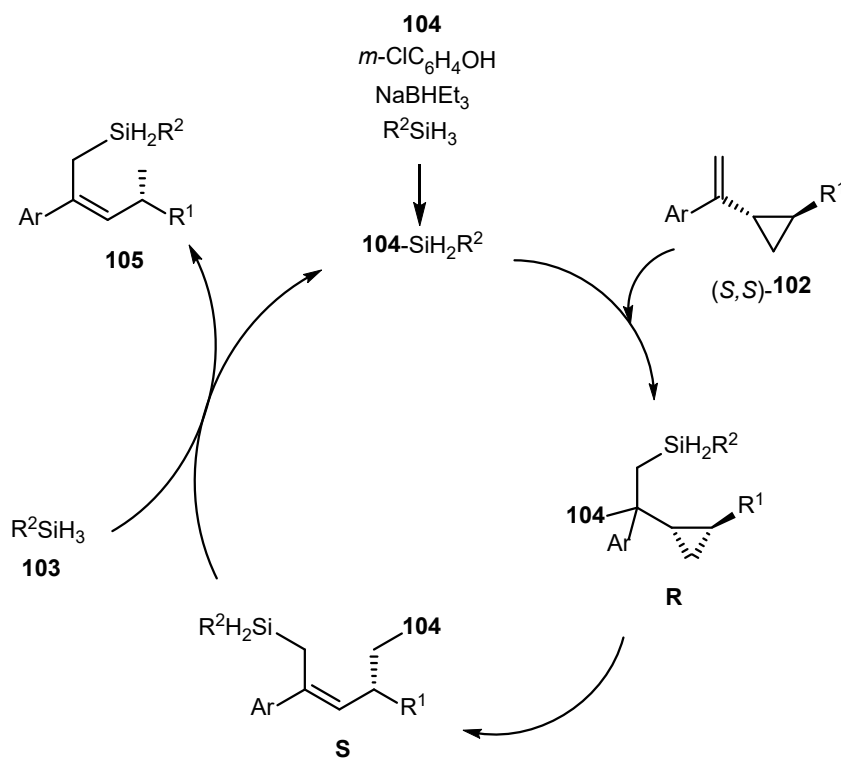
Scheme 26. Domino silylation/ring-opening reaction of vinylcyclopropanes with silanes.
