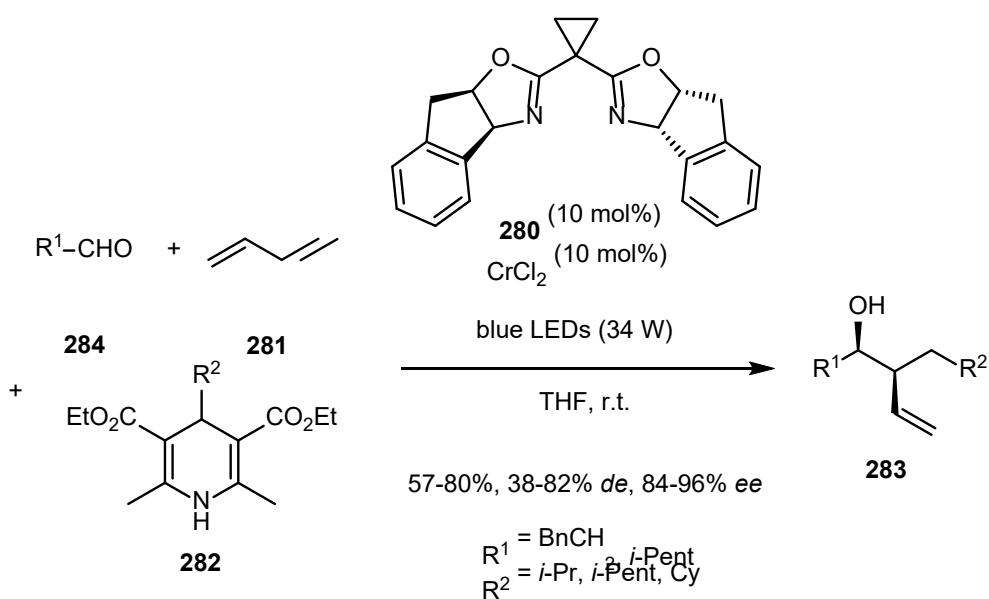
Scheme 70. Three-component domino radical dialkylation reaction of butadiene, aliphatic aldehydes and 4-alkyl Hantzsch esters.
