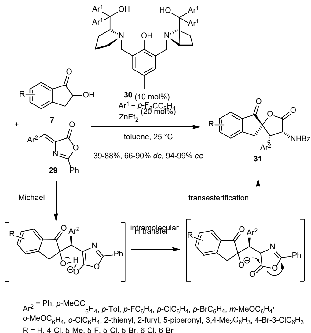
Scheme 9. Domino Michael/H-transfer/transesterification reaction of 2-hydroxy-1-indanones with alkylidene azlactones.
