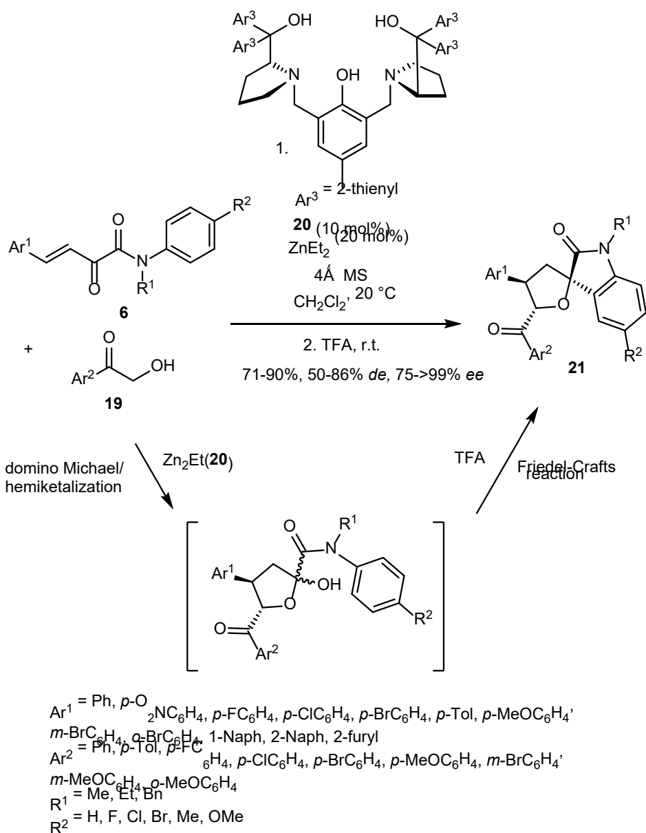
Scheme 6. Domino Michael/hemiketalization reaction of \alpha -hydroxy aryl ketones with \beta,\gamma -unsaturated \alpha -ketoamides followed by Friedel–Crafts reaction.
