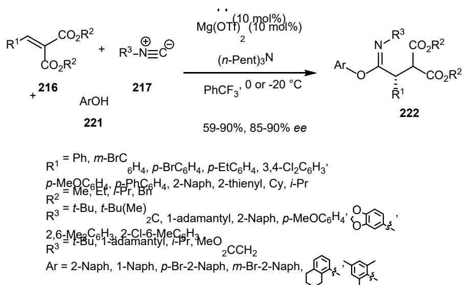
Scheme 56. Three-component reaction of alkylidene malonates, isocyanides and phenols.
