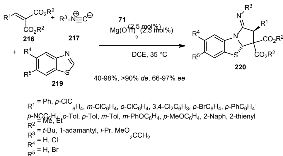
Scheme 55. Three-component domino reaction of alkylidene malonates, isocyanides and benzothiazoles.
