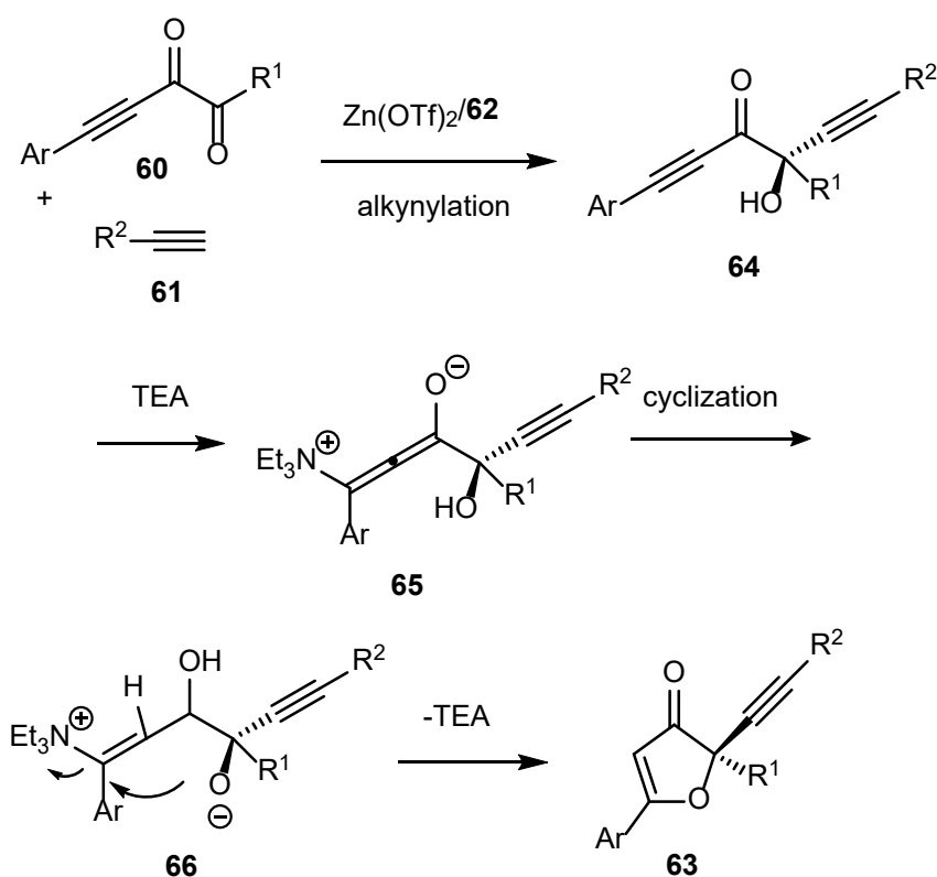
Scheme 15. Domino alkyne alkylation/cyclization reaction of alkynyl 1,2-diketones with alkynes.
