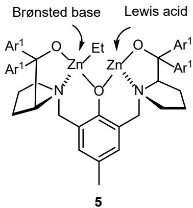
Scheme 1. Domimo phospha-Michael/Michael reaction of o -dienones with dialkyl phosphates.
