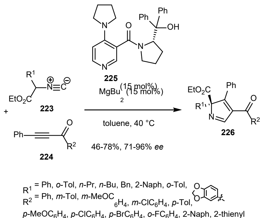
Scheme 57. Domino Michael/cyclization reaction of \alpha -isocyanoacetates with alkynyl ketones.
