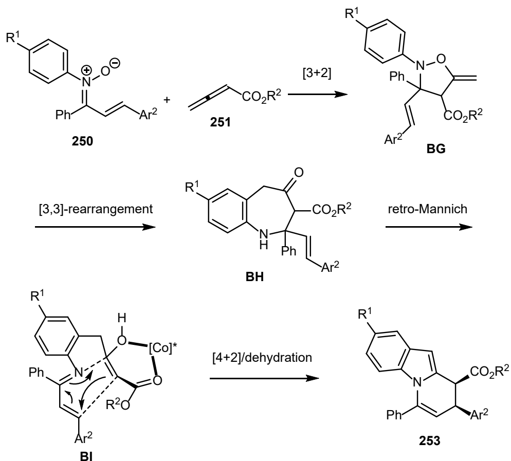
Scheme 65. Domino [3+2] cycloaddition/[3,3] rearrangement/retro-Mannich/[4+2] cycloaddition/dehydration reaction of \alpha,\beta -unsaturated- N -aryl nitrones.
