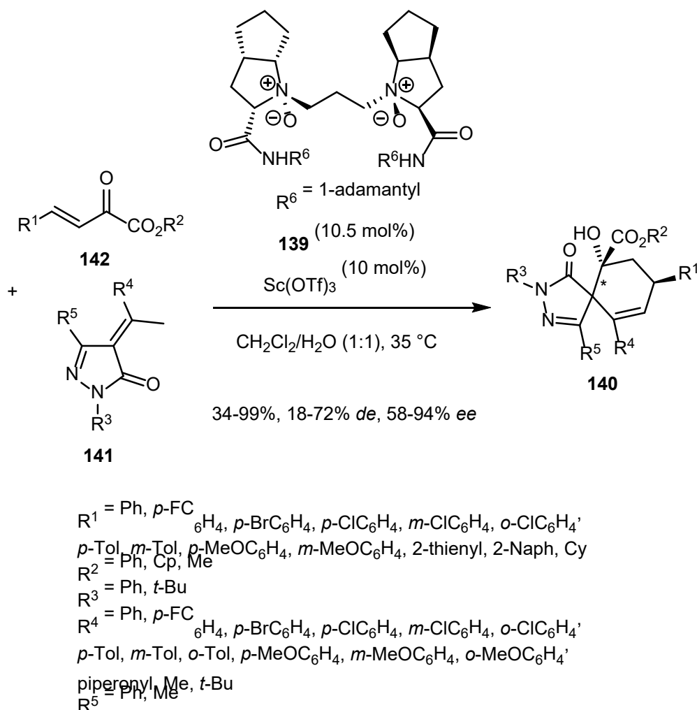
Scheme 36. Domino Michael/aldol reaction of \alpha -arylidene pyrazolinones with \beta,\gamma -unsaturated \alpha -ketoesters.
