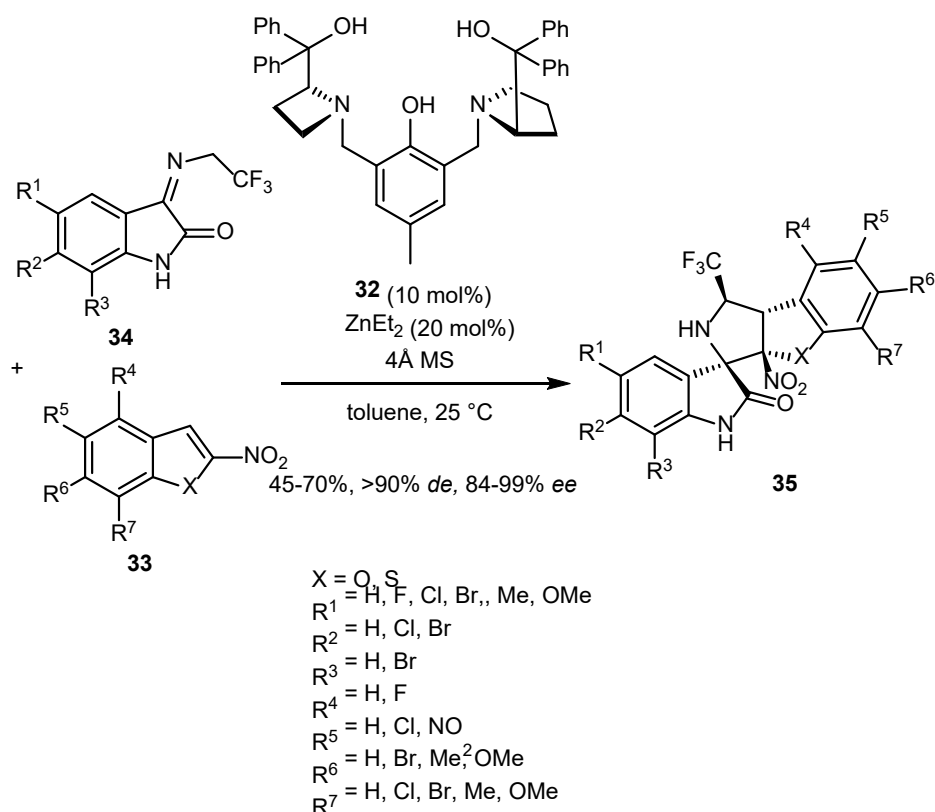
Scheme 10. Domino Michael/Mannich reaction of 2-nitrobenzofurans/2-nitrobenzothiophenes with CF_3 -containing N -unprotected isatins.
