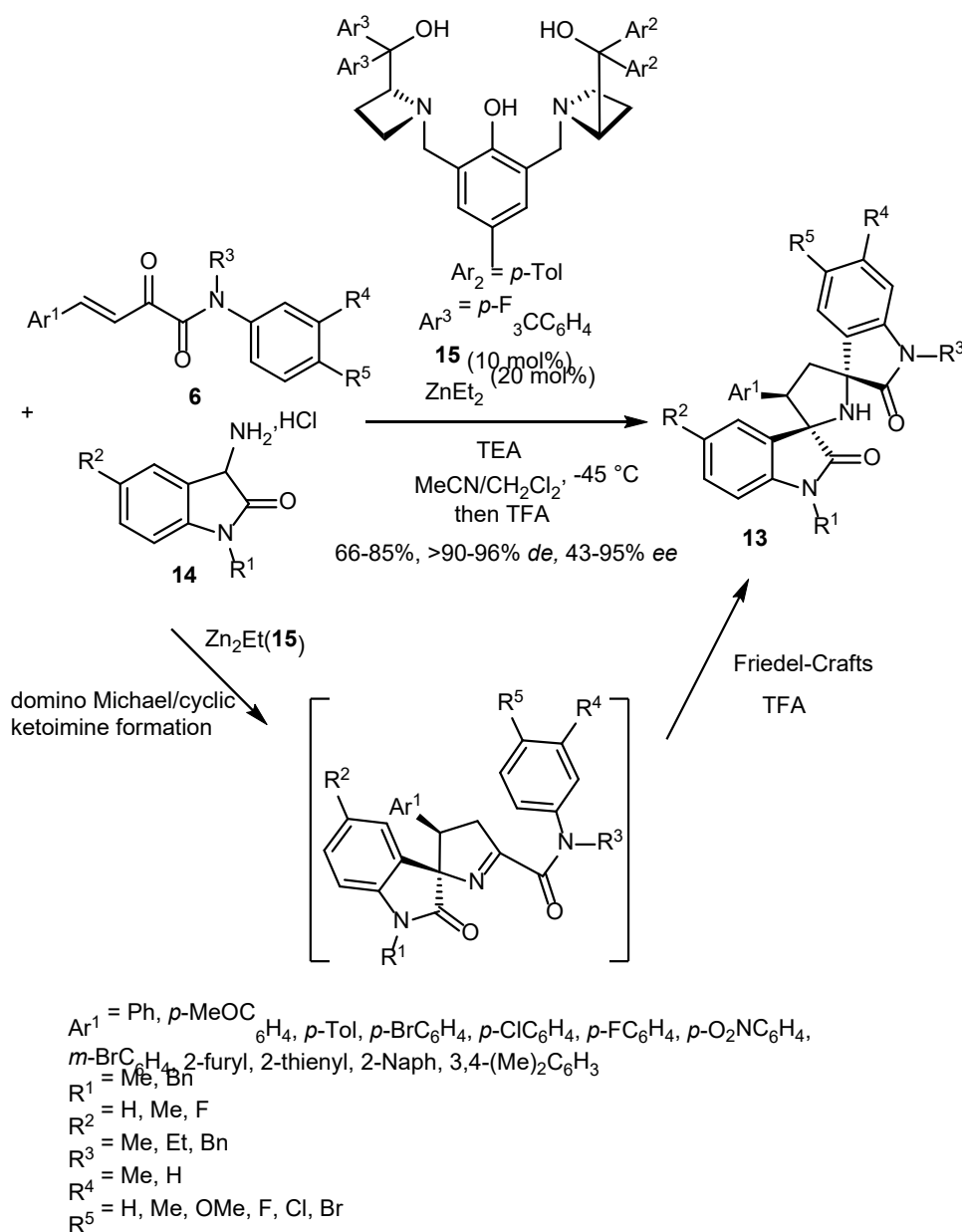
Scheme 4. Domino Michael/cyclic ketoimine formation reaction of 3-amino oxindole hydrochlorides with \beta,\gamma -unsaturated \alpha -keto amides followed by Friedel–Crafts reaction.
