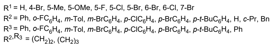
Scheme 16. Domino Friedel-Crafts/cyclization reaction of 3-aminophenols with isatylidene \alpha,\alpha -dicyanoolefins.
