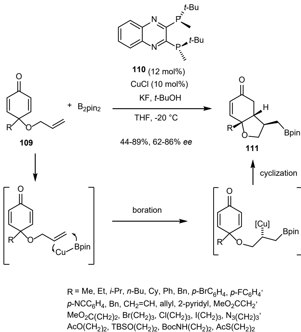
Scheme 28. Domino boration/cyclization reaction of monosubstituted terminal alkene-tethered cyclohexadienones with \text{B}_2\text{pin}_2 .
