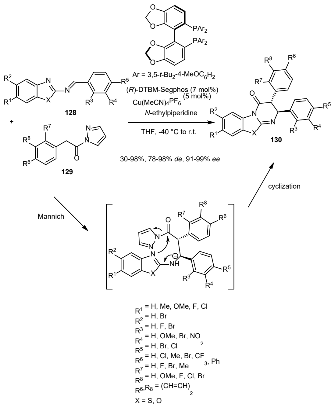
Scheme 33. Domino Mannich/cyclization reaction of 2-benzothiazolimines with N -acylpyrazoles.
