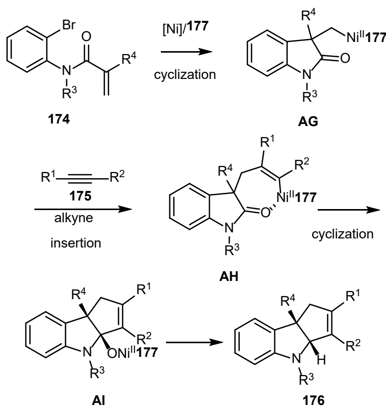
Scheme 44. Domino reductive cyclization reaction of alkene-tethered aryl bromides with internal alkynes.
