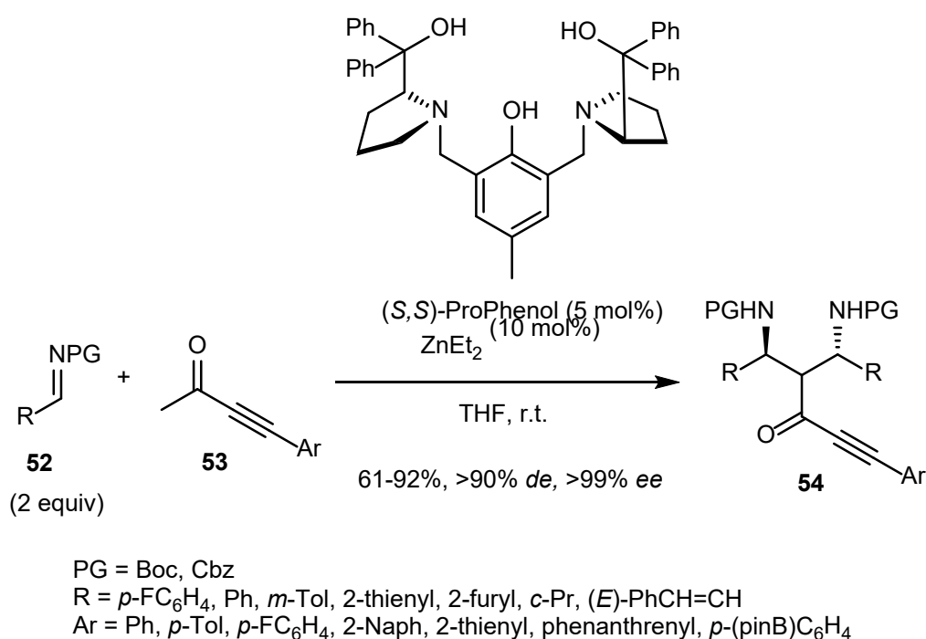
Scheme 13. Pseudo-three-component domino double Mannich reaction of ynones with aldimines.
