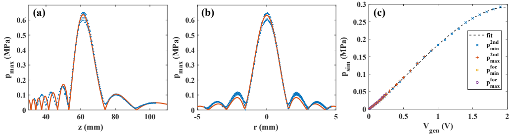
Figure 6: Evolution of the maximum acoustic pressure in the axial (a) and radial (b) direction at low amplitude. The red lines correspond to the prediction of the acoustic simulation using the non-linear code (Soneson 2009), while the blue dots represent the experimental points. (c) Evolution of the input pressure of the simulation ( p_{\text{sim}} ) fitting the different maximum and minimum measurements as a function of the generator voltage ( V_{\text{gen}} ).
