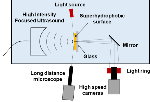
Figure 1: Schematic of the experimental setup. Short acoustic pulses are emitted by a High Intensity Focused Ultrasound transducer and focused upon the tested surface held by a glass coverslip. The dynamic is monitored from the side and from the bottom by two high speed cameras.
