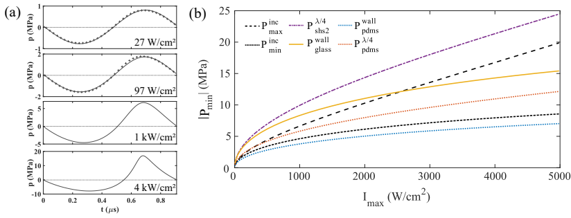
Figure 4: (a) Incident waveform at the focal plan for different maximum incident intensity ( I_{max} ). The simulation results (solid lines) using the nonlinear acoustic code (Soneson 2009) are compared to the experimental measurements (cross points) at low intensity. (b) Evolution of the minimum and maximum incident pressure ( P_{min,max}^{inc} ) and of the minimum local pressure ( P_{min}^{position, surface} ) at specific position for a surface with the maximum incident intensity ( I_{max} ).
