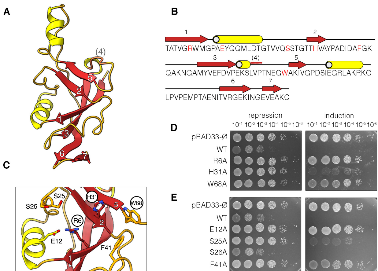
Figure 2. Tre Tu structure. (A) Ribbon representation of the S. enterica Tre Tu domain. The \beta -strands, including the pseudo- \beta -strand \beta_4 , are numbered. (B) Secondary structures of Tre Tu . The putative residues involved in NAD + binding and catalysis are colored by element. (C) Magnification of the enzymatic pocket highlighting the residues involved in NAD + binding and catalysis. (D and E) Toxicity assay in the heterologous host E. coli . Cultures of E. coli cells producing the Tre Tu toxin and its variants from the pBAD33rbs vector were serially diluted and spotted on LB-agar plates supplemented with 1% glucose (repression conditions, left panel) or 0.2% L-arabinose (induction conditions, right panel). Effect of mutations in the putative catalytic triad is shown in (D), and further residues suggested to be involved in NAD + binding and catalysis are shown in (E).
