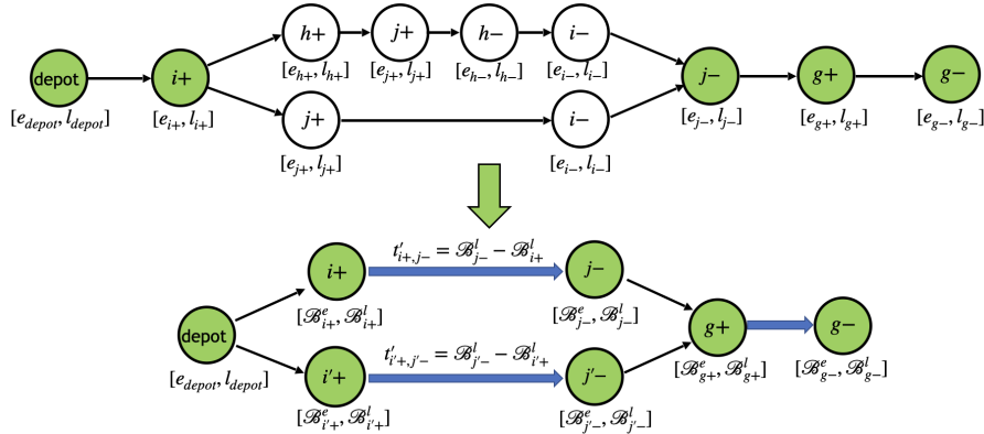
FIG. 1 – Example of constructing arcs in the new graph G_{sp}
