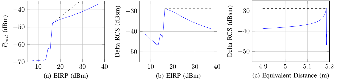
Fig. 9. (a) Differential backscattered power as a function of the EIRP. (b) Delta RCS as a function of the EIRP. (c) Delta RCS as a function of the equivalent distance. All curves have been measured at 915 MHz.
