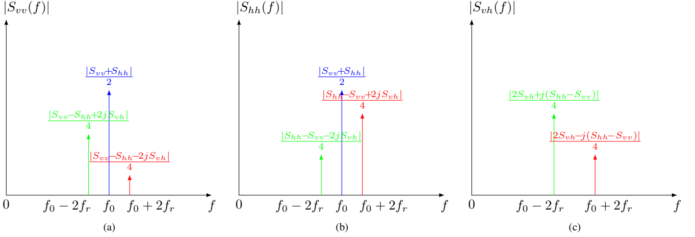
Fig. 2. Unilateral spectrum of a rotating tag at f_r , impinged by a CW at f_0 in (a) vertical co-polarization [see (8a)], (b) horizontal co-polarization [see (8b)] and (c) cross-polarization [see (8c)].
